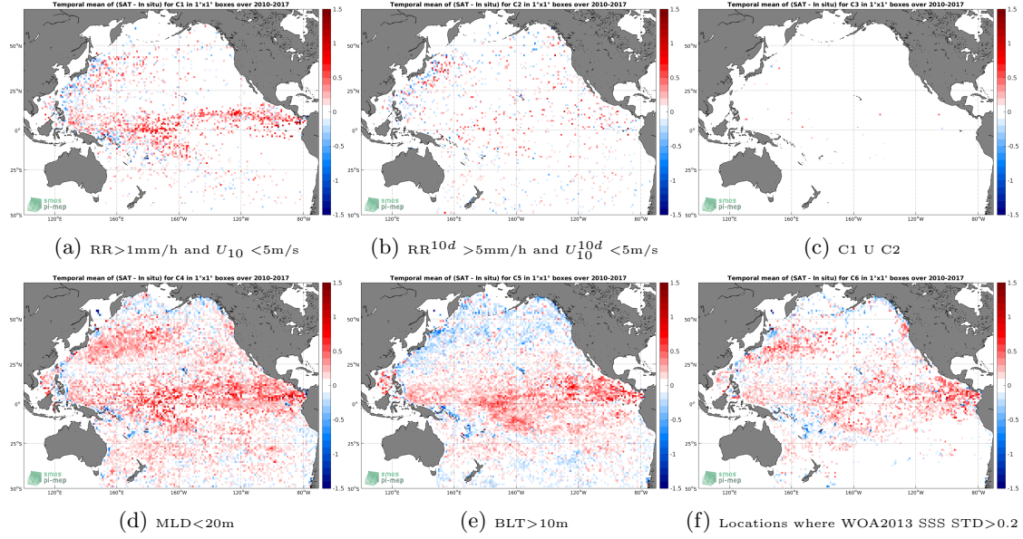
Figure 12: Temporal mean gridded over spatial boxes of size 1^\circ \times 1^\circ of \Delta\text{SSS} (SMOS-L3-BEC-OA-V1-9DAYS-0.25DEG - Argo) for 6 different subdatasets corresponding to: RR > 1\text{mm/h} and U_{10} < 5\text{m/s} (a), RR^{10d} > 5\text{mm/h} and U_{10}^{10d} < 5\text{m/s} (b), C1 U C2 (c), MLD < 20\text{m} (d), BLT > 10\text{m} (e), Locations where WOA2013 SSS STD > 0.2 (f).
