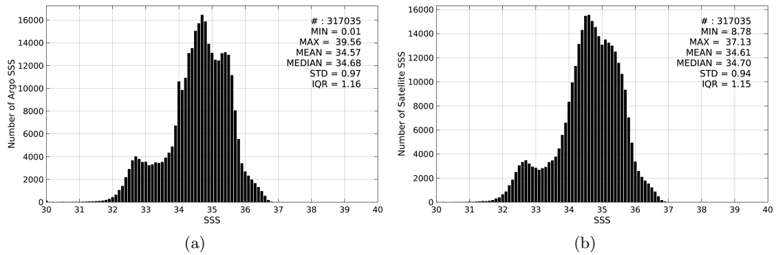
Figure 2: Histograms of SSS from Argo (a) and SMOS-L3-BEC-OA-V1-9DAYS-0.25DEG (b) considering all match-up pairs per bins of 0.1 over the Pacific Ocean Pi-MEP region and for the full satellite product period.
