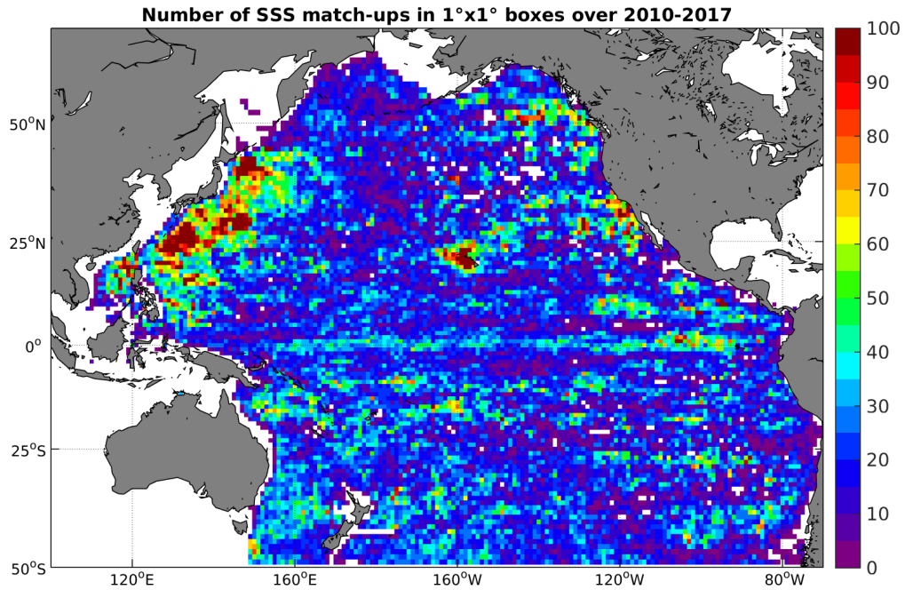
Figure 4: Number of SSS match-ups between Argo SSS and the SMOS-L3-BEC-OA-V1-9DAYS-0.25DEG SSS product for the Pacific Ocean Pi-MEP region over 1^\circ \times 1^\circ boxes and for the full satellite product period.
