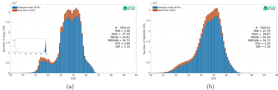
Figure 2: Histograms of SSS from Argo (a) and SMOS SSS L2-AVERAGED v700 (ESA) (b) considering all match-up pairs per bins of 0.1 over the Pacific Ocean Pi-MEP region and for the full satellite product period.
