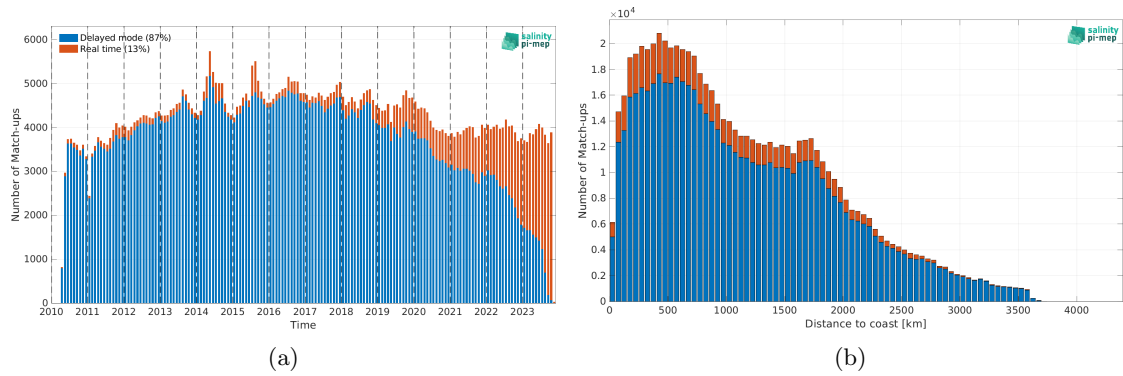
Figure 1: Number of match-ups between Argo and SMOS SSS L2-AVERAGED v700 (ESA) SSS as a function of time (a) and as function of the distance to coast (b) over the Pacific Ocean Pi-MEP region and for the full satellite product period.
