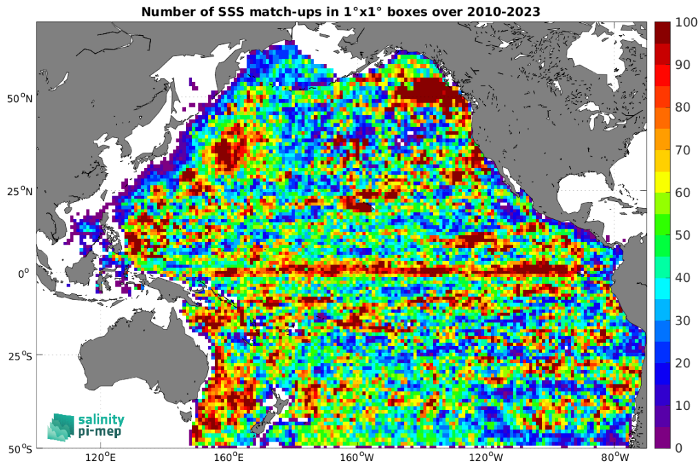
Figure 4: Number of SSS match-ups between Argo SSS and the SMOS SSS L2-AVERAGED v700 (ESA) SSS product for the Pacific Ocean Pi-MEP region over 1^\circ \times 1^\circ boxes and for the full satellite product period.
