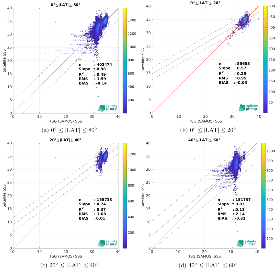
Figure 9: Contour maps of the concentration of SMOS SSS L2 v700 (ESA) SSS (y-axis) versus TSG (SAMOS) SSS (x-axis) at match-up pairs for different latitude bands. For each plot, the red line shows x=y . The black thin and dashed lines indicate a linear fit through the data cloud and the \pm 95\% confidence levels, respectively. The number match-up pairs n , the slope and R^2 coefficient of the linear fit, the root mean square (RMS) and the mean bias between satellite and in situ data are indicated for each latitude band in each plots.
