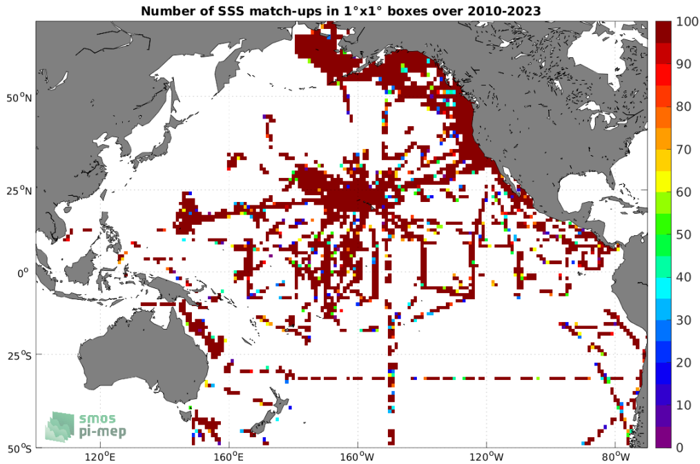
Figure 4: Number of SSS match-ups between TSG (SAMOS) SSS and the SMOS SSS L2 v700 (ESA) SSS product for the Pacific Ocean Pi-MEP region over 1^\circ \times 1^\circ boxes and for the full satellite product period.
