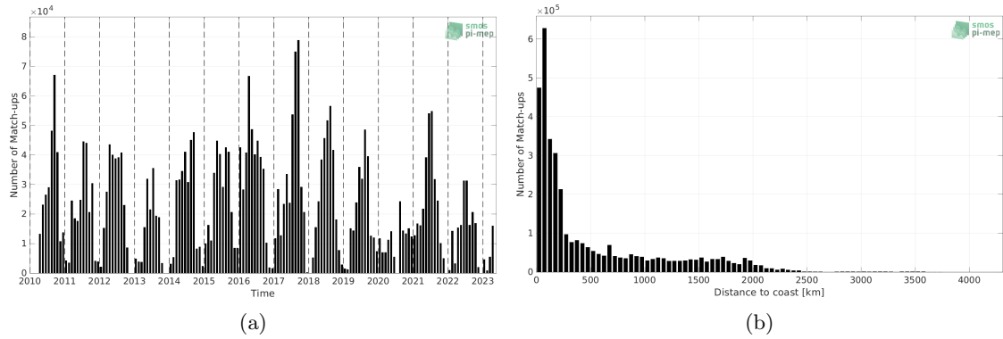
Figure 1: Number of match-ups between TSG (SAMOS) and SMOS SSS L2 v700 (ESA) SSS as a function of time (a) and as function of the distance to coast (b) over the Pacific Ocean Pi-MEP region and for the full satellite product period.
