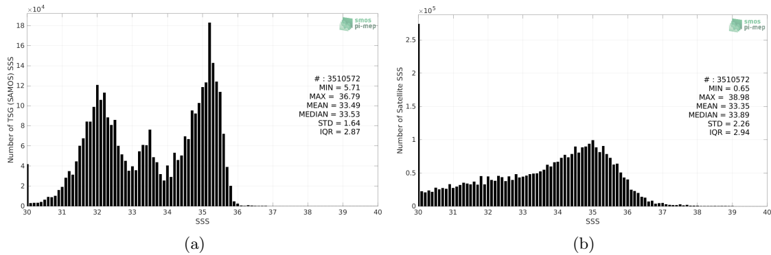
Figure 2: Histograms of SSS from TSG (SAMOS) (a) and SMOS SSS L2 v700 (ESA) (b) considering all match-up pairs per bins of 0.1 over the Pacific Ocean Pi-MEP region and for the full satellite product period.
