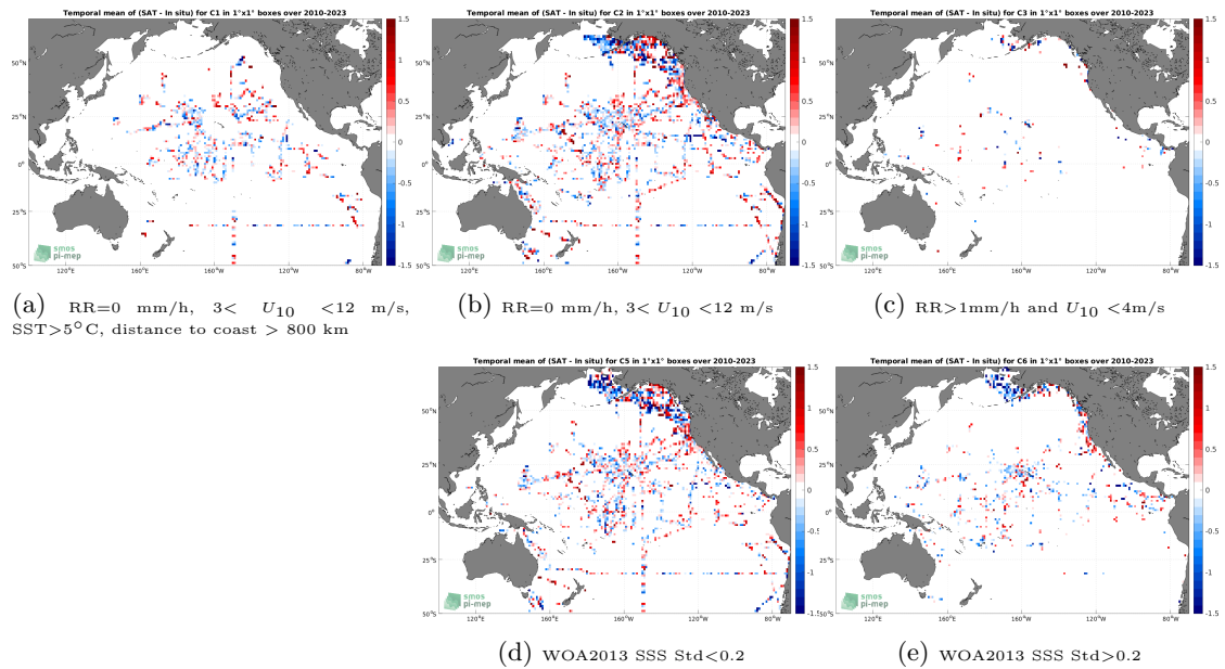
Figure 12: Temporal mean gridded over spatial boxes of size 1^\circ \times 1^\circ of \Delta SSS (SMOS SSS L2 v700 (ESA) - TSG (SAMOS)) for 5 different subdatasets corresponding to:RR=0 mm/h, 3 < U_{10} < 12 m/s, SST > 5^\circ\text{C} , distance to coast > 800 km (a), RR=0 mm/h, 3 < U_{10} < 12 m/s (b), RR > 1 mm/h and U_{10} < 4 m/s (c), WOA2013 SSS Std < 0.2 (d), WOA2013 SSS Std > 0.2 (e).
