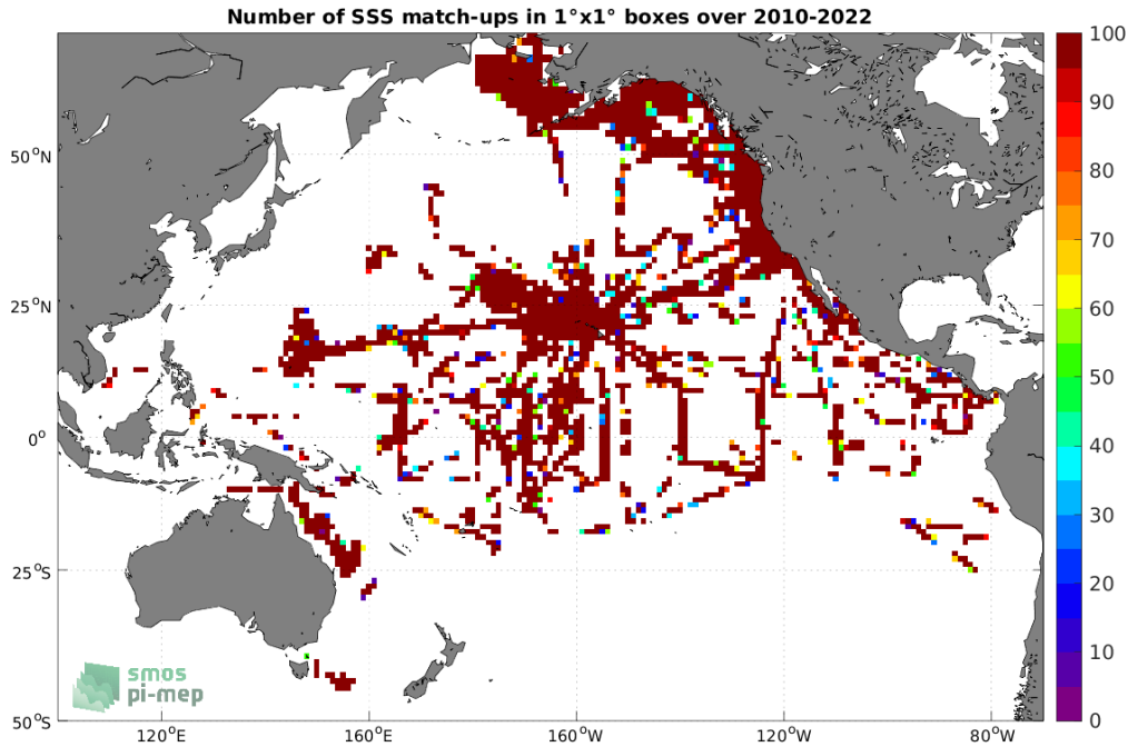
Figure 4: Number of SSS match-ups between TSG (SAMOS) SSS and the SMOS SSS L2 v700 (ESA) SSS product for the Pacific Ocean Pi-MEP region over 1°x1° boxes and for the full satellite product period.
