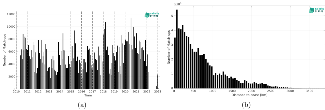
Figure 2: Number of match-ups between TSG (LEGOS-DM) and SMOS SSS L2 v700 (ESA) SSS as a function of time (a) and as function of the distance to coast (b) over the Pacific Ocean Pi-MEP region and for the full satellite product period.
