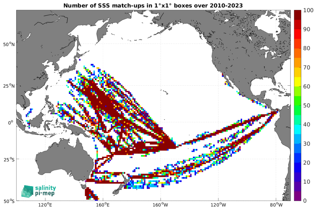
Figure 5: Number of SSS match-ups between TSG (LEGOS-DM) SSS and the SMOS SSS L2 v700 (ESA) SSS product for the Pacific Ocean Pi-MEP region over 1^\circ \times 1^\circ boxes and for the full satellite product period.
