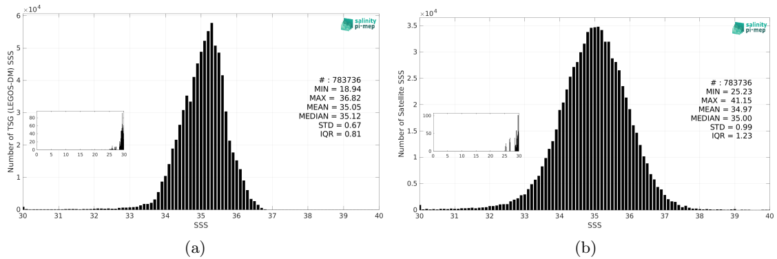
Figure 3: Histograms of SSS from TSG (LEGOS-DM) (a) and SMOS SSS L2 v700 (ESA) (b) considering all match-up pairs per bins of 0.1 over the Pacific Ocean Pi-MEP region and for the full satellite product period.
