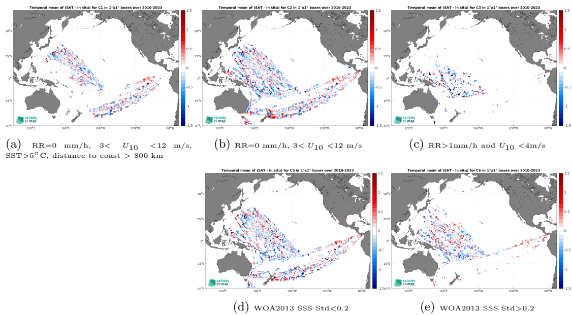
Figure 14: Temporal mean gridded over spatial boxes of size 1^\circ \times 1^\circ of \Delta SSS (SMOS SSS L2 v700 (ESA) - TSG (LEGOS-DM)) for 5 different subdatasets corresponding to: RR=0 mm/h, 3 < U_{10} < 12 m/s, SST > 5°C, distance to coast > 800 km (a), RR=0 mm/h, 3 < U_{10} < 12 m/s (b), RR > 1mm/h and U_{10} < 4 m/s (c), WOA2013 SSS Std < 0.2 (d), WOA2013 SSS Std > 0.2 (e).
