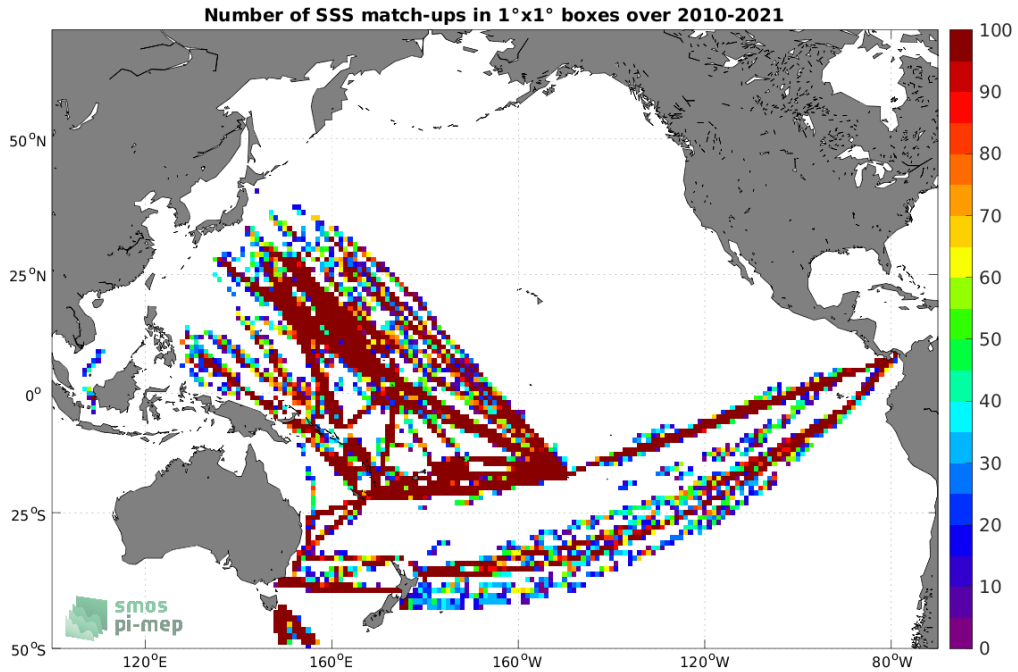
Figure 4: Number of SSS match-ups between TSG (LEGOS-DM) SSS and the SMOS SSS L2 v700 (ESA) SSS product for the Pacific Ocean Pi-MEP region over 1^\circ \times 1^\circ boxes and for the full satellite product period.
