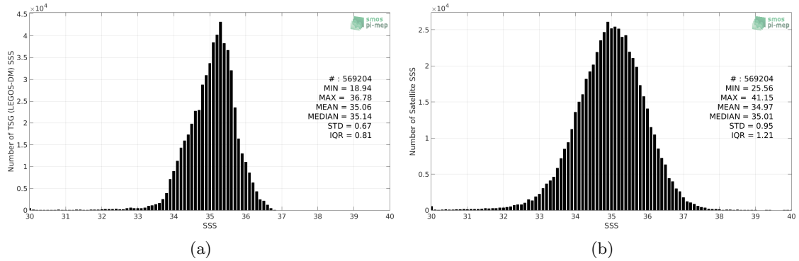
Figure 2: Histograms of SSS from TSG (LEGOS-DM) (a) and SMOS SSS L2 v700 (ESA) (b) considering all match-up pairs per bins of 0.1 over the Pacific Ocean Pi-MEP region and for the full satellite product period.
