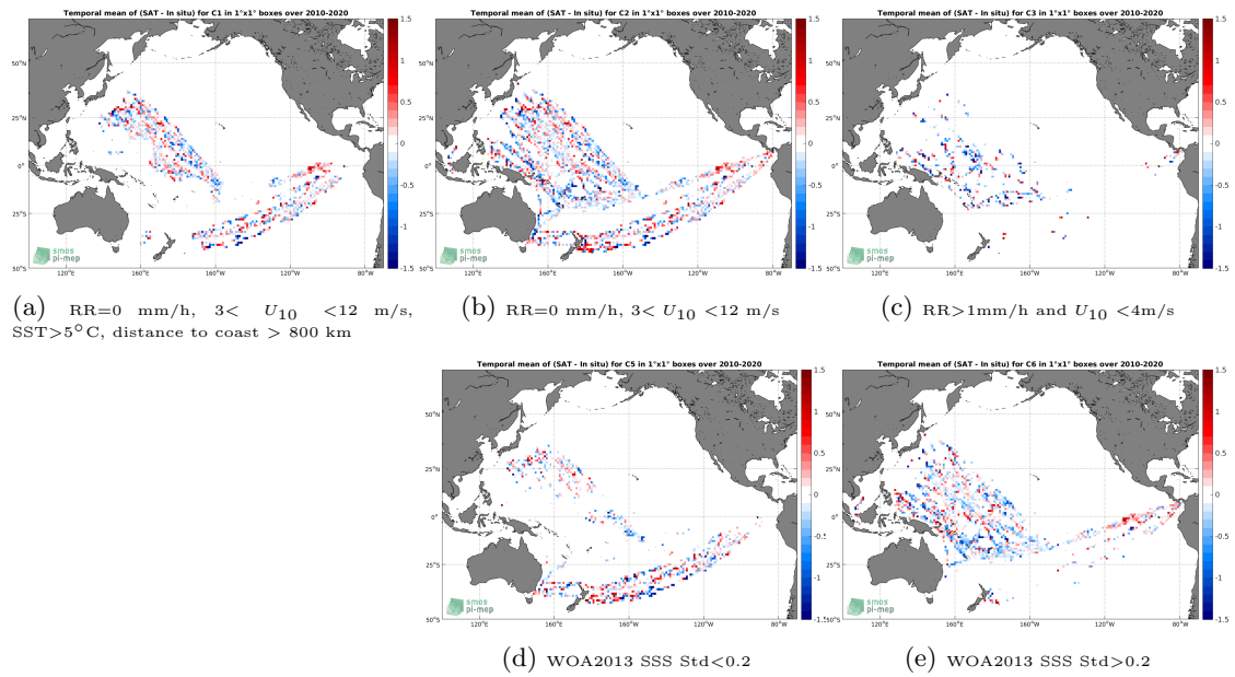
Figure 12: Temporal mean gridded over spatial boxes of size 1^\circ \times 1^\circ of \Delta SSS (SMOS SSS L2 v700 (ESA) - TSG (LEGOS-DM)) for 5 different subdatasets corresponding to: RR=0 mm/h, 3 < U_{10} < 12 m/s, SST > 5°C, distance to coast > 800 km (a), RR=0 mm/h, 3 < U_{10} < 12 m/s (b), RR > 1mm/h and U_{10} < 4 m/s (c), WOA2013 SSS Std < 0.2 (d), WOA2013 SSS Std > 0.2 (e).
