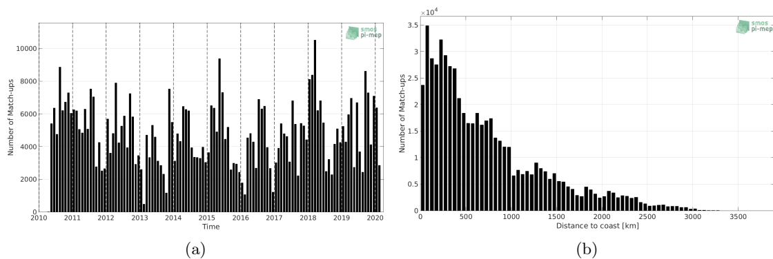
Figure 1: Number of match-ups between TSG (LEGOS-DM) and SMOS SSS L2 v700 (ESA) SSS as a function of time (a) and as function of the distance to coast (b) over the Pacific Ocean Pi-MEP region and for the full satellite product period.
