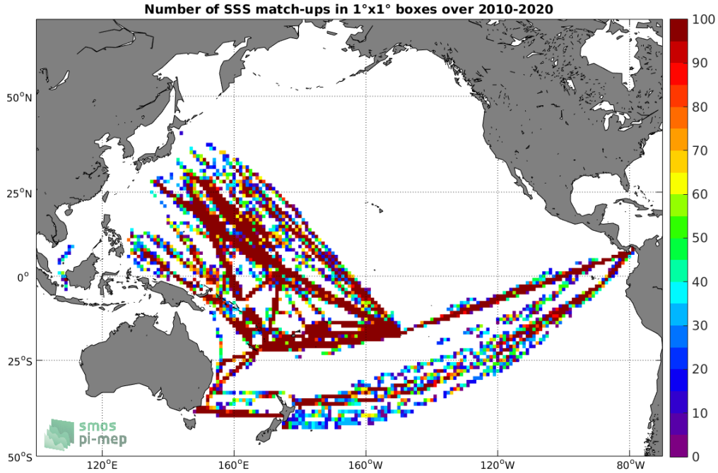
Figure 4: Number of SSS match-ups between TSG (LEGOS-DM) SSS and the SMOS SSS L2 v700 (ESA) SSS product for the Pacific Ocean Pi-MEP region over 1°x1° boxes and for the full satellite product period.
