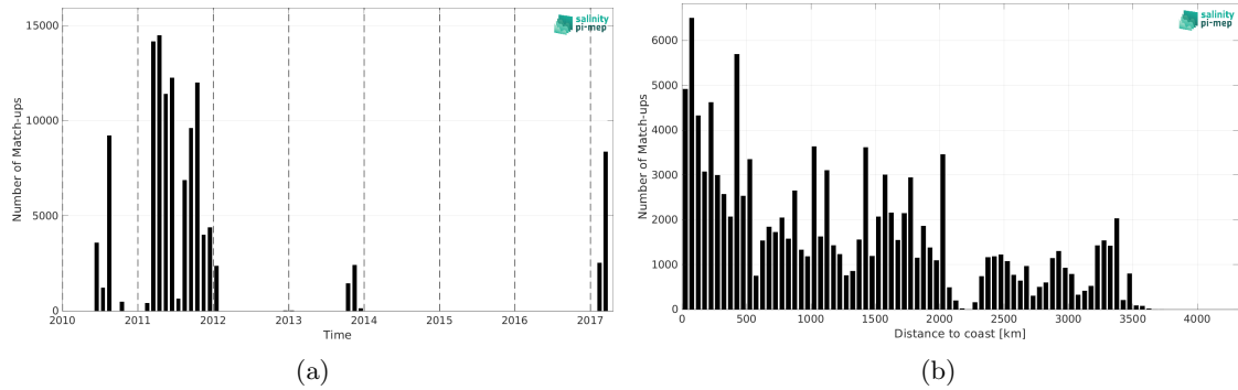
Figure 2: Number of match-ups between TSG (GOSUD-Sailing-ship) and SMOS SSS L2 v700 (ESA) SSS as a function of time (a) and as function of the distance to coast (b) over the Pacific Ocean Pi-MEP region and for the full satellite product period.
