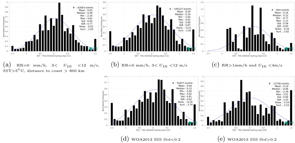
Figure 15: Normalized histogram of \Delta SSS (SMOS SSS L2 v700 (ESA) - TSG (GOSUD-Sailing-ship)) for 5 different subdatasets corresponding to: RR=0 mm/h, 3 < U_{10} < 12 m/s, SST>5°C, distance to coast > 800 km (a), RR=0 mm/h, 3 < U_{10} < 12 m/s (b), RR>1mm/h and U_{10} < 4 m/s (c), WOA2013 SSS Std<0.2 (d), WOA2013 SSS Std>0.2 (e).
