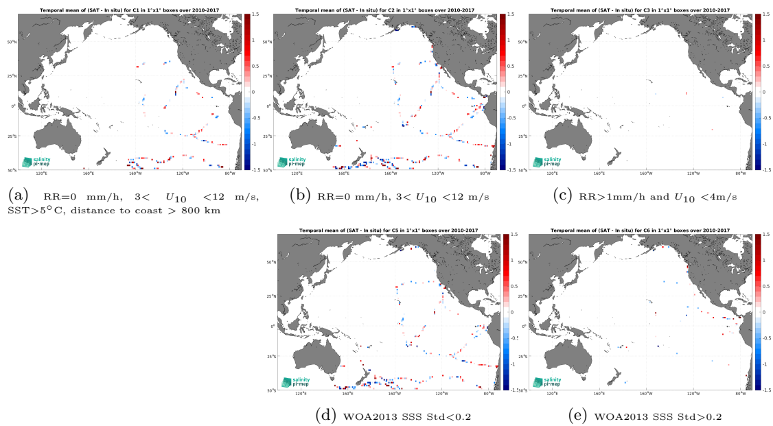
Figure 14: Temporal mean gridded over spatial boxes of size 1^\circ \times 1^\circ of \Delta SSS (SMOS SSS L2 v700 (ESA) - TSG (GOSUD-Sailing-ship)) for 5 different subdatasets corresponding to: RR=0 mm/h, 3 < U_{10} < 12 m/s, SST > 5^\circ C , distance to coast > 800 km (a), RR=0 mm/h, 3 < U_{10} < 12 m/s (b), RR > 1mm/h and U_{10} < 4 m/s (c), WOA2013 SSS Std < 0.2 (d), WOA2013 SSS Std > 0.2 (e).
