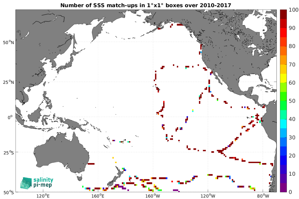
Figure 5: Number of SSS match-ups between TSG (GOSUD-Sailing-ship) SSS and the SMOS SSS L2 v700 (ESA) SSS product for the Pacific Ocean Pi-MEP region over 1^\circ \times 1^\circ boxes and for the full satellite product period.
