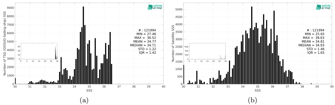
Figure 3: Histograms of SSS from TSG (GOSUD-Sailing-ship) (a) and SMOS SSS L2 v700 (ESA) (b) considering all match-up pairs per bins of 0.1 over the Pacific Ocean Pi-MEP region and for the full satellite product period.
