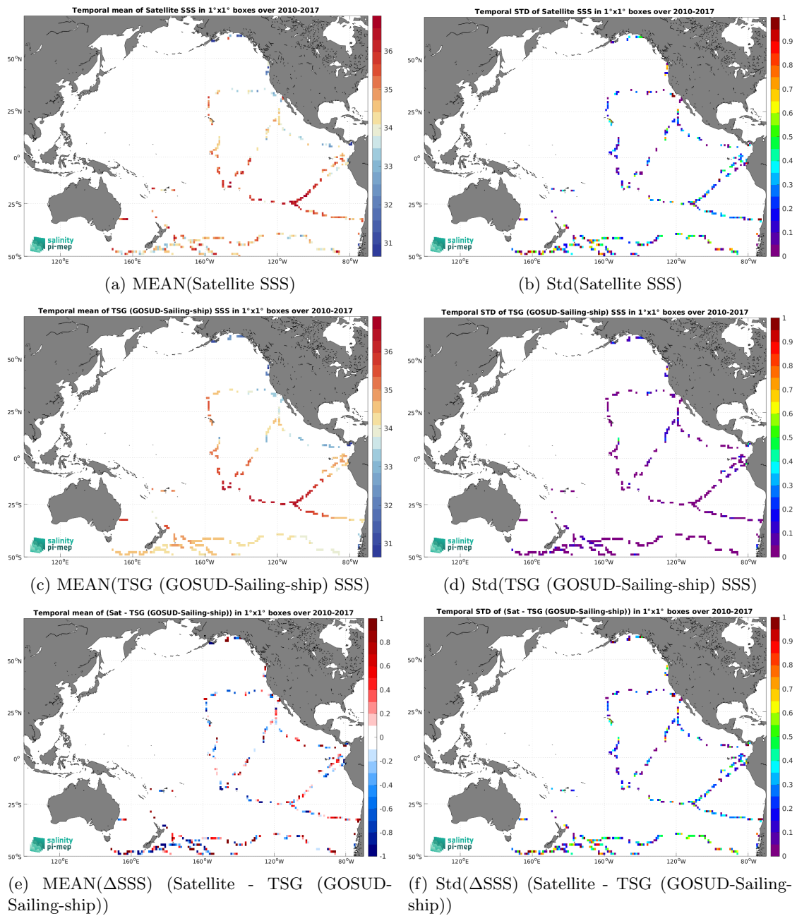
Figure 7: Temporal mean (left) and Std (right) of SSS from SMOS SSS L2 v700 (ESA) (top), TSG (GOSUD-Sailing-ship) (middle), and of \Delta SSS (Satellite - TSG (GOSUD-Sailing-ship)). Only match-up pairs are used to generate these maps.
