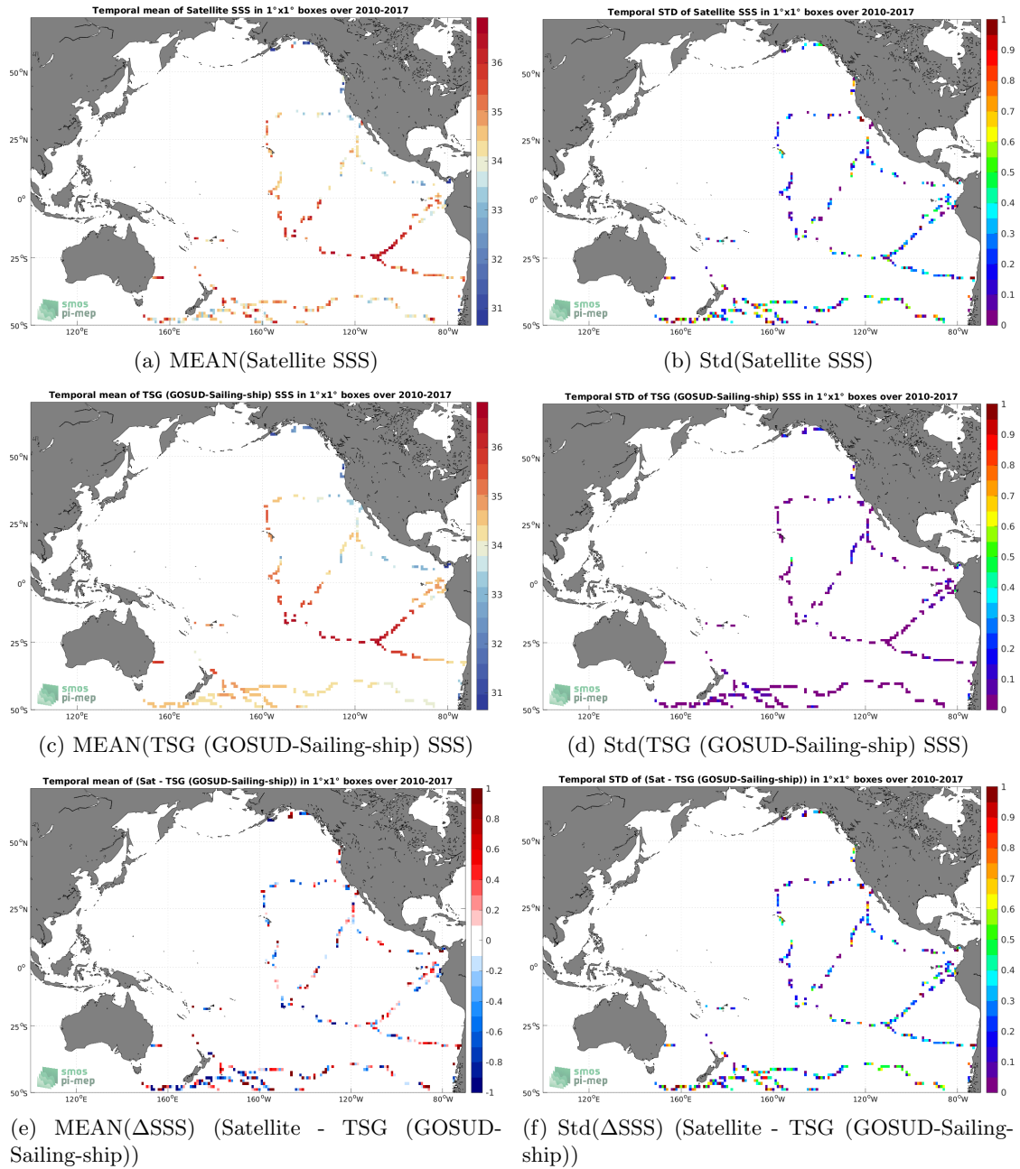
Figure 6: Temporal mean (left) and Std (right) of SSS from SMOS SSS L2 v700 (ESA) (top), TSG (GOSUD-Sailing-ship) (middle), and of \Delta SSS (Satellite - TSG (GOSUD-Sailing-ship)). Only match-up pairs are used to generate these maps.
