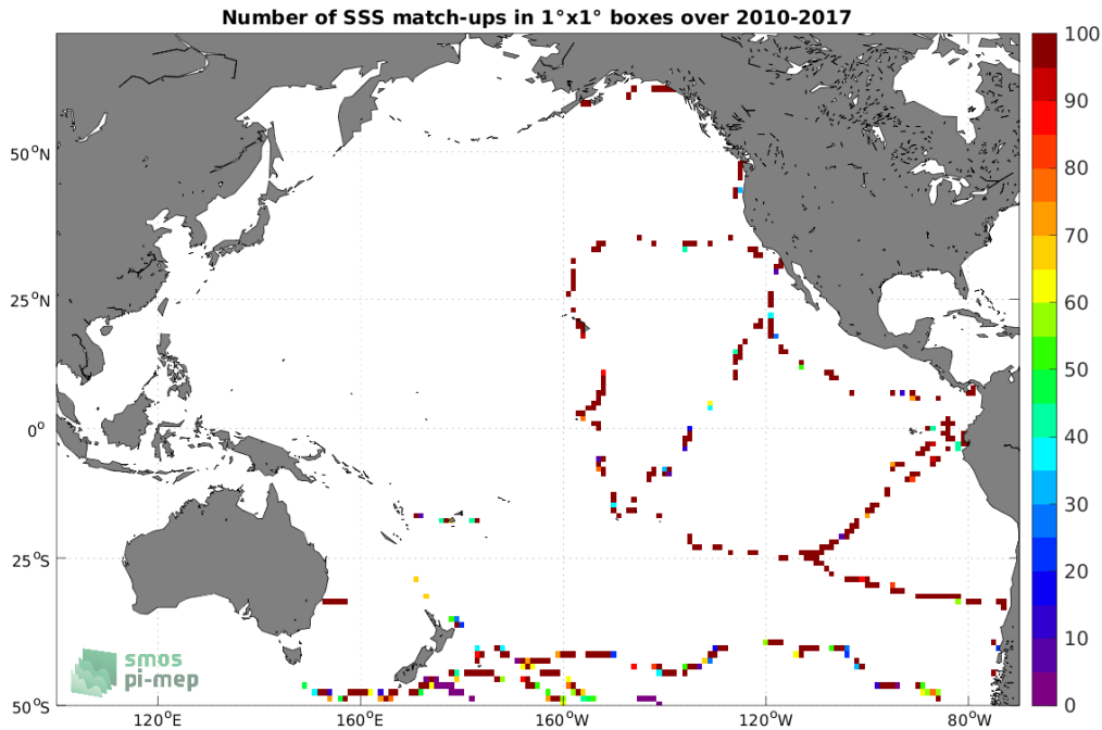
Figure 4: Number of SSS match-ups between TSG (GOSUD-Sailing-ship) SSS and the SMOS SSS L2 v700 (ESA) SSS product for the Pacific Ocean Pi-MEP region over 1^\circ \times 1^\circ boxes and for the full satellite product period.
