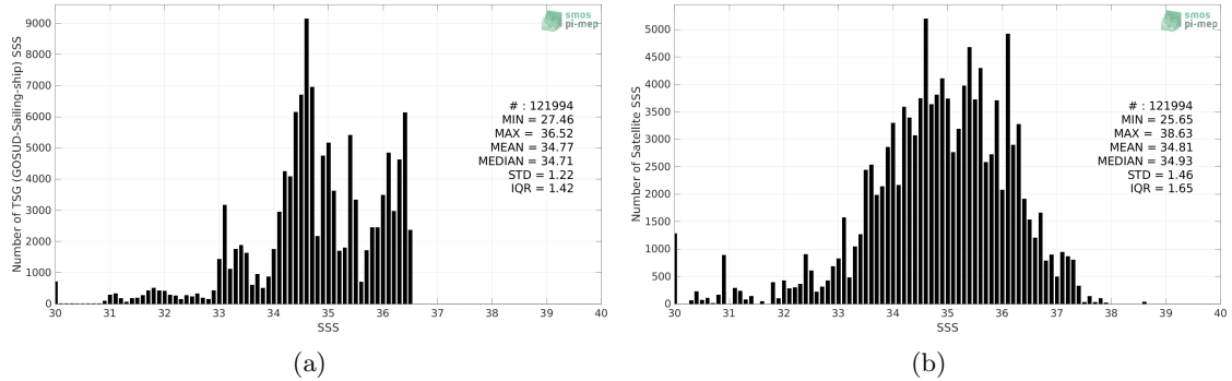
Figure 2: Histograms of SSS from TSG (GOSUD-Sailing-ship) (a) and SMOS SSS L2 v700 (ESA) (b) considering all match-up pairs per bins of 0.1 over the Pacific Ocean Pi-MEP region and for the full satellite product period.
