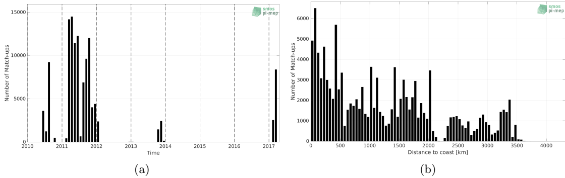
Figure 1: Number of match-ups between TSG (GOSUD-Sailing-ship) and SMOS SSS L2 v700 (ESA) SSS as a function of time (a) and as function of the distance to coast (b) over the Pacific Ocean Pi-MEP region and for the full satellite product period.
