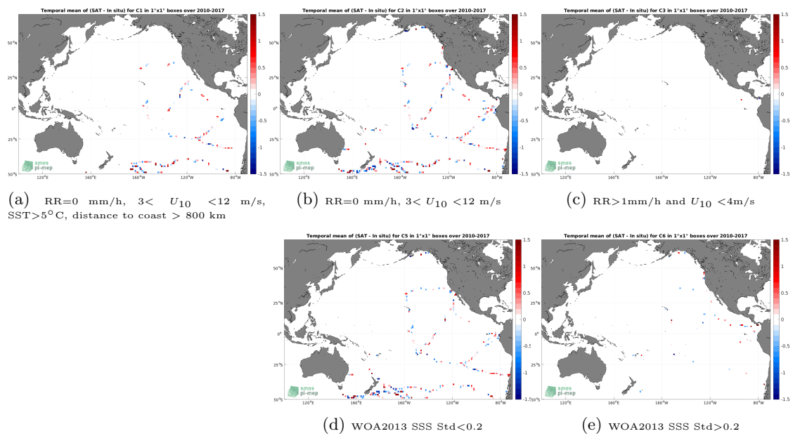
Figure 12: Temporal mean gridded over spatial boxes of size 1^\circ \times 1^\circ of \Delta SSS (SMOS SSS L2 v700 (ESA) - TSG (GOSUD-Sailing-ship)) for 5 different subdatasets corresponding to: RR=0 mm/h, 3 < U_{10} < 12 m/s, SST > 5°C, distance to coast > 800 km (a), RR=0 mm/h, 3 < U_{10} < 12 m/s (b), RR > 1mm/h and U_{10} < 4 m/s (c), WOA2013 SSS Std < 0.2 (d), WOA2013 SSS Std > 0.2 (e).
