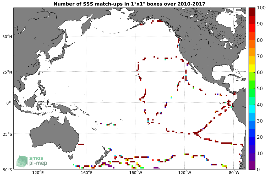
Figure 4: Number of SSS match-ups between TSG (GOSUD-Sailing-ship) SSS and the SMOS SSS L2 v700 (ESA) SSS product for the Pacific Ocean Pi-MEP region over 1°x1° boxes and for the full satellite product period.
