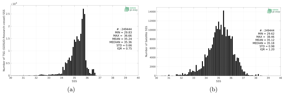
Figure 2: Histograms of SSS from TSG (GOSUD-Research-vessel) (a) and SMOS SSS L2 v700 (ESA) (b) considering all match-up pairs per bins of 0.1 over the Pacific Ocean Pi-MEP region and for the full satellite product period.
