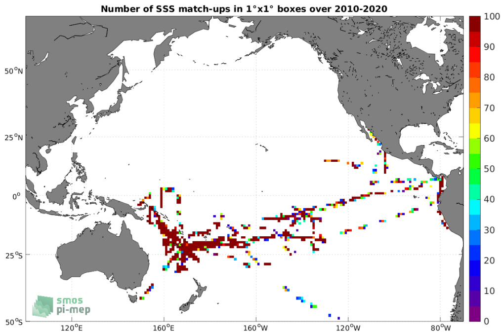
Figure 4: Number of SSS match-ups between TSG (GOSUD-Research-vessel) SSS and the SMOS SSS L2 v700 (ESA) SSS product for the Pacific Ocean Pi-MEP region over 1^\circ \times 1^\circ boxes and for the full satellite product period.
