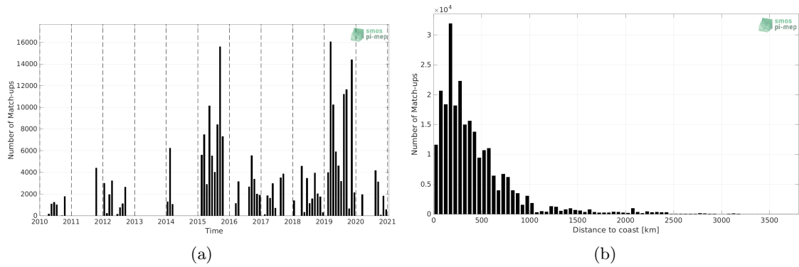
Figure 1: Number of match-ups between TSG (GOSUD-Research-vessel) and SMOS SSS L2 v700 (ESA) SSS as a function of time (a) and as function of the distance to coast (b) over the Pacific Ocean Pi-MEP region and for the full satellite product period.
