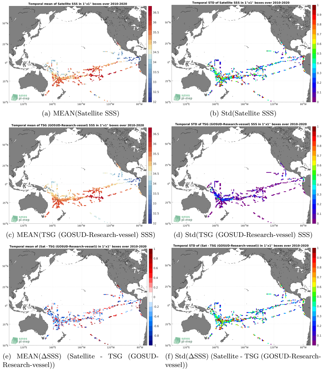
Figure 6: Temporal mean (left) and Std (right) of SSS from SMOS SSS L2 v700 (ESA) (top), TSG (GOSUD-Research-vessel) (middle), and of \Delta SSS (Satellite - TSG (GOSUD-Research-vessel)). Only match-up pairs are used to generate these maps.
