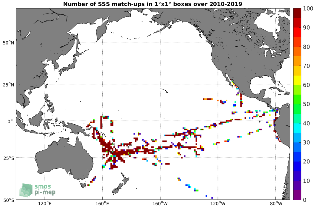
Figure 4: Number of SSS match-ups between TSG (GOSUD-Research-vessel) SSS and the SMOS SSS L2 v700 (ESA) SSS product for the Pacific Ocean Pi-MEP region over 1°x1° boxes and for the full satellite product period.
