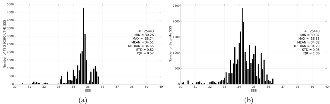
Figure 3: Histograms of SSS from TSG (CSIC-UTM) (a) and SMOS SSS L2 v700 (ESA) (b) considering all match-up pairs per bins of 0.1 over the Pacific Ocean Pi-MEP region and for the full satellite product period.
