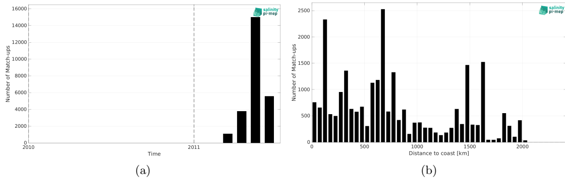
Figure 2: Number of match-ups between TSG (CSIC-UTM) and SMOS SSS L2 v700 (ESA) SSS as a function of time (a) and as function of the distance to coast (b) over the Pacific Ocean Pi-MEP region and for the full satellite product period.
