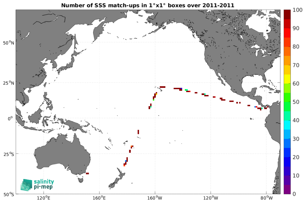
Figure 5: Number of SSS match-ups between TSG (CSIC-UTM) SSS and the SMOS SSS L2 v700 (ESA) SSS product for the Pacific Ocean Pi-MEP region over 1^\circ \times 1^\circ boxes and for the full satellite product period.
