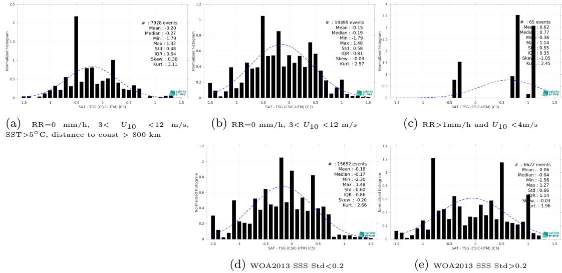
Figure 13: Normalized histogram of \Delta\text{SSS} (SMOS SSS L2 v700 (ESA) - TSG (CSIC-UTM)) for 5 different subdatasets corresponding to: RR=0 mm/h, 3 < U_{10} < 12 m/s, SST>5°C, distance to coast > 800 km (a), RR=0 mm/h, 3 < U_{10} < 12 m/s (b), RR>1mm/h and U_{10} < 4 m/s (c), WOA2013 SSS Std<0.2 (d), WOA2013 SSS Std>0.2 (e).
