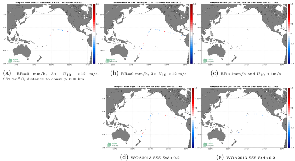
Figure 12: Temporal mean gridded over spatial boxes of size 1^\circ \times 1^\circ of \Delta SSS (SMOS SSS L2 v700 (ESA) - TSG (CSIC-UTM)) for 5 different subdatasets corresponding to:RR=0 mm/h, 3 < U_{10} < 12 m/s, SST >5^\circ C, distance to coast > 800 km (a), RR=0 mm/h, 3 < U_{10} < 12 m/s (b), RR >1 mm/h and U_{10} < 4 m/s (c), WOA2013 SSS Std <0.2 (d), WOA2013 SSS Std >0.2 (e).
