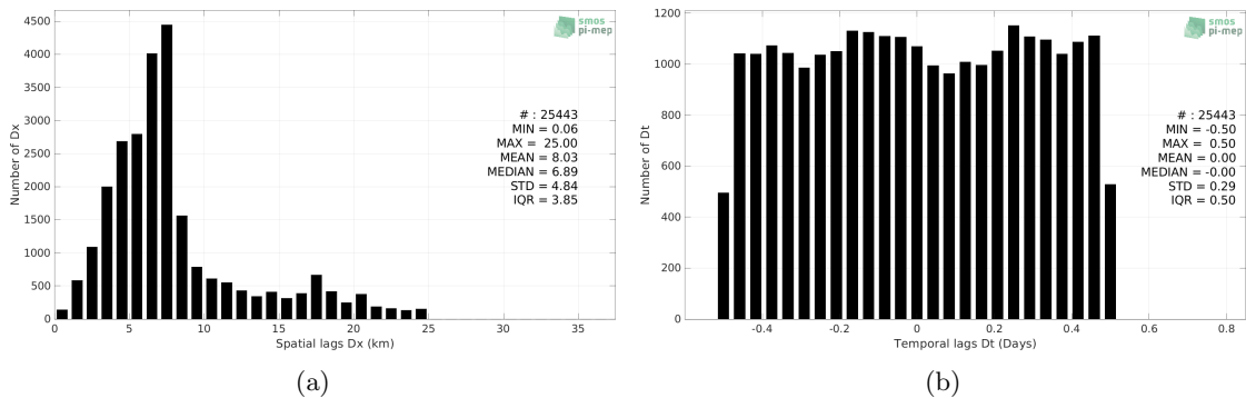
Figure 5: Histograms of the spatial (a) and temporal (b) lags between the location/time of the TSG (CSIC-UTM) measurement and the date of the corresponding SMOS SSS L2 v700 (ESA) SSS pixel.
