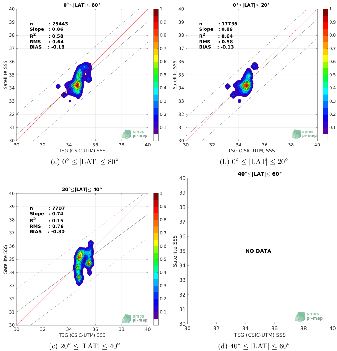
Figure 9: Contour maps of the concentration of SMOS SSS L2 v700 (ESA) SSS (y-axis) versus TSG (CSIC-UTM) SSS (x-axis) at match-up pairs for different latitude bands. For each plot, the red line shows x=y . The black thin and dashed lines indicate a linear fit through the data cloud and the \pm 95\% confidence levels, respectively. The number match-up pairs n , the slope and R^2 coefficient of the linear fit, the root mean square (RMS) and the mean bias between satellite and in situ data are indicated for each latitude band in each plots.
