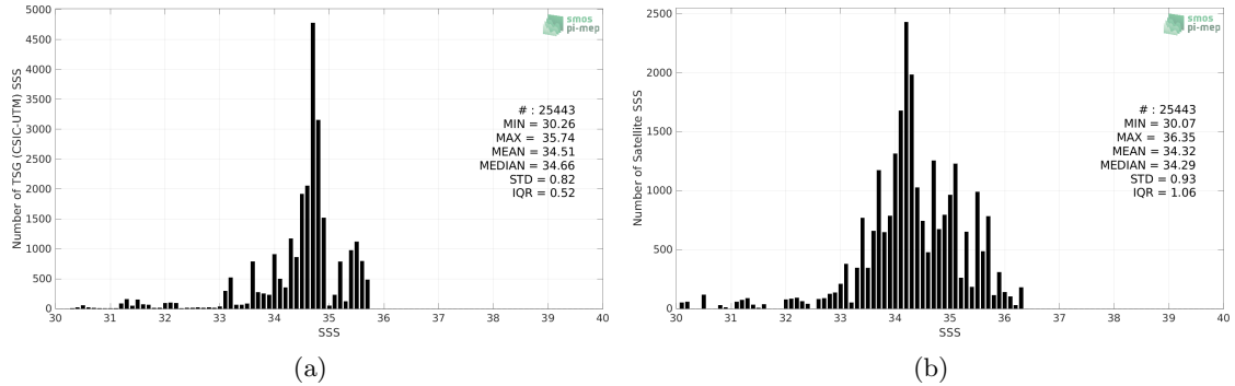
Figure 2: Histograms of SSS from TSG (CSIC-UTM) (a) and SMOS SSS L2 v700 (ESA) (b) considering all match-up pairs per bins of 0.1 over the Pacific Ocean Pi-MEP region and for the full satellite product period.
