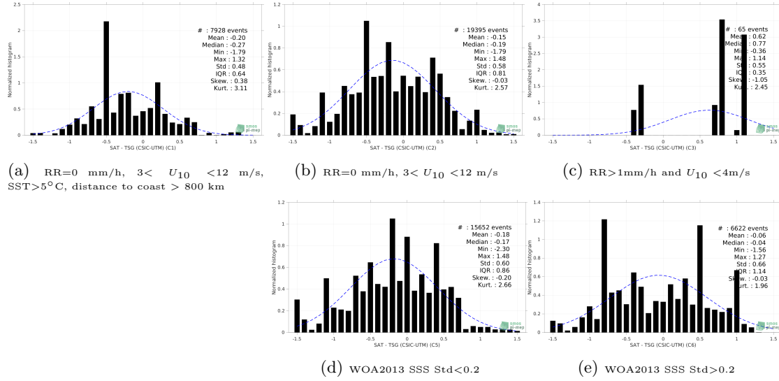
Figure 13: Normalized histogram of \Delta SSS (SMOS SSS L2 v700 (ESA) - TSG (CSIC-UTM)) for 5 different subdatasets corresponding to: RR=0 mm/h, 3 < U_{10} < 12 m/s, SST > 5°C, distance to coast > 800 km (a), RR=0 mm/h, 3 < U_{10} < 12 m/s (b), RR > 1mm/h and U_{10} < 4 m/s (c), WOA2013 SSS Std < 0.2 (d), WOA2013 SSS Std > 0.2 (e).
