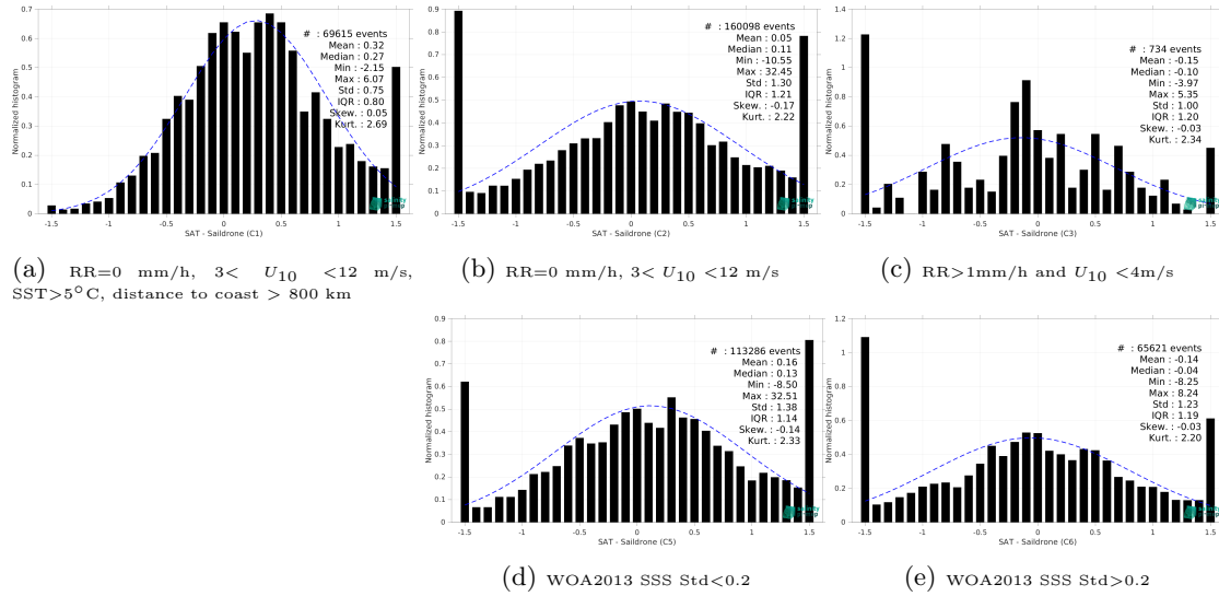
Figure 15: Normalized histogram of \Delta SSS (SMOS SSS L2 v700 (ESA) - Salldrone) for 5 different subdatasets corresponding to: RR=0 mm/h, 3 < U_{10} < 12 m/s, SST > 5°C, distance to coast > 800 km (a), RR=0 mm/h, 3 < U_{10} < 12 m/s (b), RR > 1mm/h and U_{10} < 4 m/s (c), WOA2013 SSS Std < 0.2 (d), WOA2013 SSS Std > 0.2 (e).
