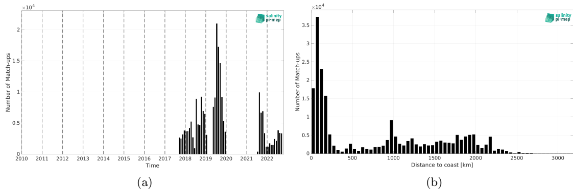
Figure 1: Number of match-ups between Saildrone and SMOS SSS L2 v700 (ESA) SSS as a function of time (a) and as function of the distance to coast (b) over the Pacific Ocean Pi-MEP region and for the full satellite product period.
