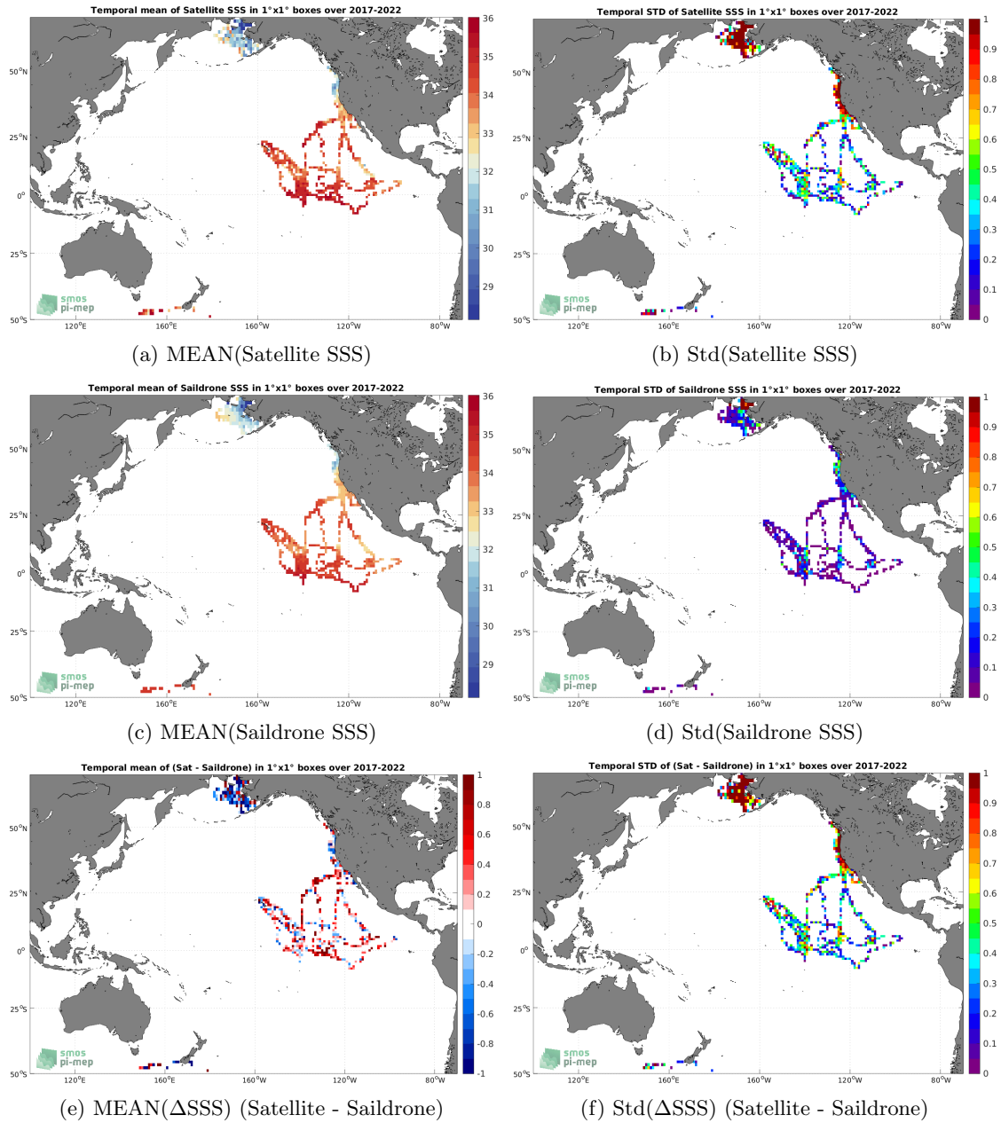
Figure 6: Temporal mean (left) and Std (right) of SSS from SMOS SSS L2 v700 (ESA) (top), Saildrone (middle), and of \Delta SSS (Satellite - Saildrone). Only match-up pairs are used to generate these maps.
