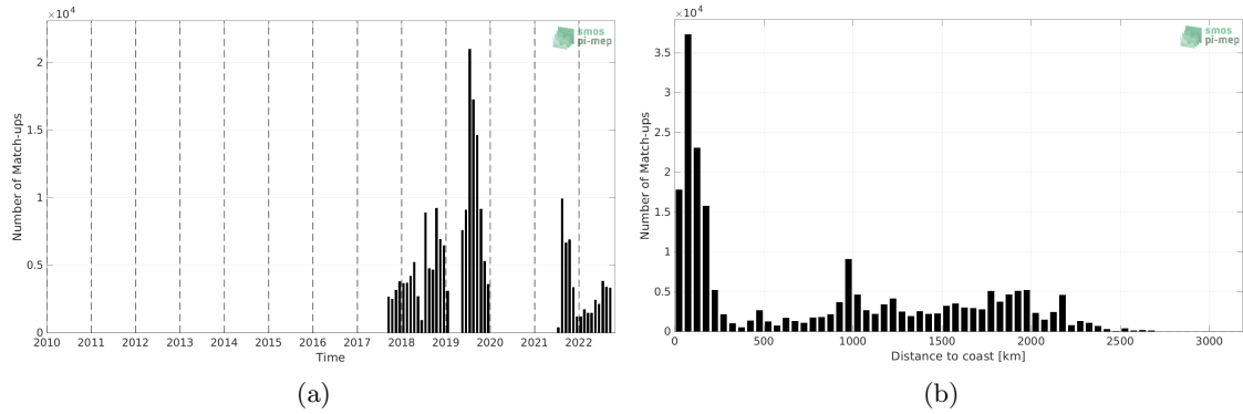
Figure 1: Number of match-ups between Sairdrone and SMOS SSS L2 v700 (ESA) SSS as a function of time (a) and as function of the distance to coast (b) over the Pacific Ocean Pi-MEP region and for the full satellite product period.
