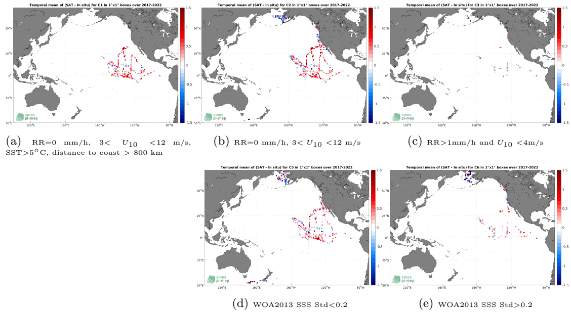
Figure 12: Temporal mean gridded over spatial boxes of size 1^\circ \times 1^\circ of \Delta SSS (SMOS SSS L2 v700 (ESA) - Sairdrone) for 5 different subdatasets corresponding to:RR=0 mm/h, 3 < U_{10} < 12 m/s, SST >5^\circ C, distance to coast > 800 km (a), RR=0 mm/h, 3 < U_{10} < 12 m/s (b), RR >1 mm/h and U_{10} < 4 m/s (c), WOA2013 SSS Std <0.2 (d), WOA2013 SSS Std >0.2 (e).
