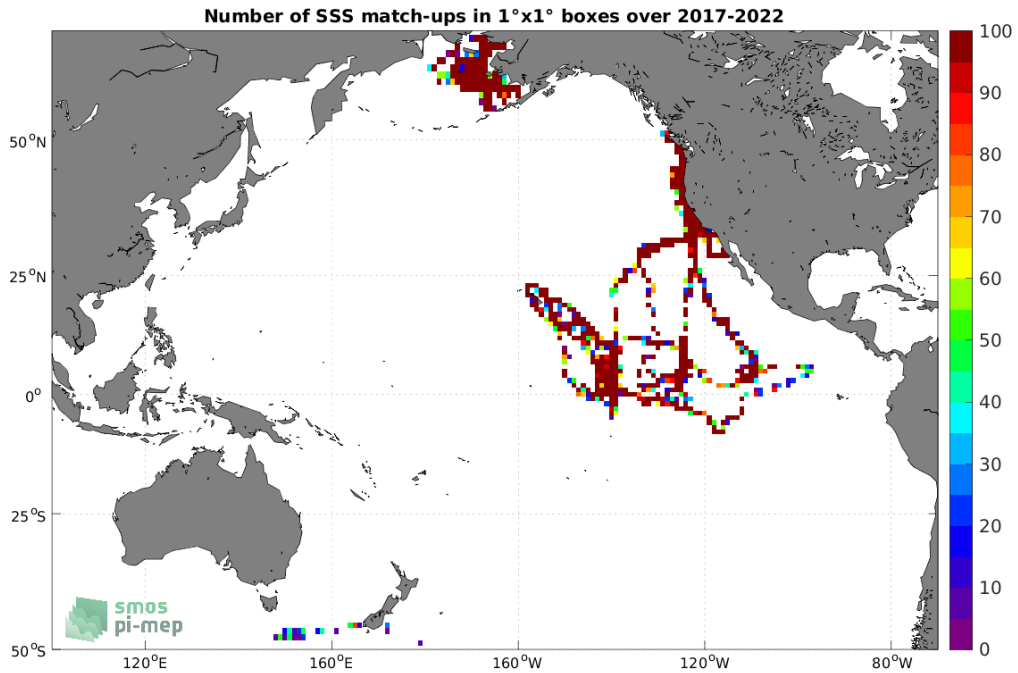
Figure 4: Number of SSS match-ups between Saildrone SSS and the SMOS SSS L2 v700 (ESA) SSS product for the Pacific Ocean Pi-MEP region over 1^\circ \times 1^\circ boxes and for the full satellite product period.
