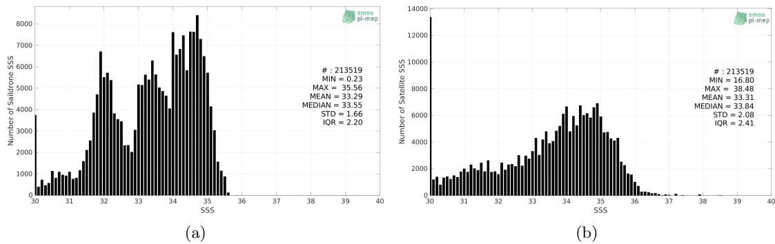
Figure 2: Histograms of SSS from Sairdrone (a) and SMOS SSS L2 v700 (ESA) (b) considering all match-up pairs per bins of 0.1 over the Pacific Ocean Pi-MEP region and for the full satellite product period.
