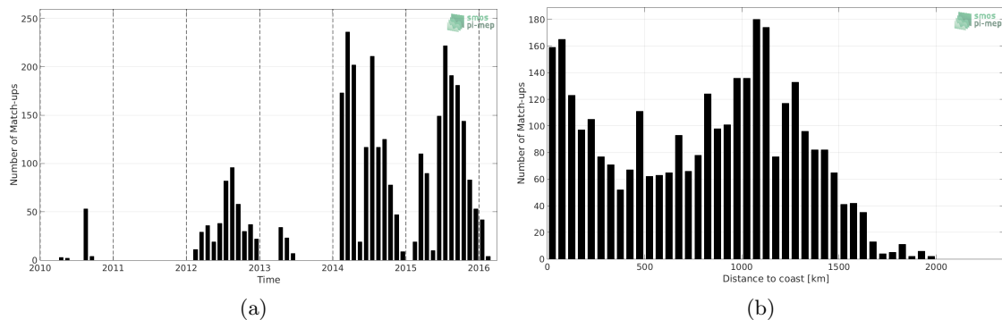
Figure 1: Number of match-ups between Sea mammals and SMOS SSS L2 v700 (ESA) SSS as a function of time (a) and as function of the distance to coast (b) over the Pacific Ocean Pi-MEP region and for the full satellite product period.
