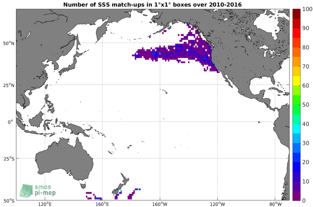
Figure 4: Number of SSS match-ups between Sea mammals SSS and the SMOS SSS L2 v700 (ESA) SSS product for the Pacific Ocean Pi-MEP region over 1°x1° boxes and for the full satellite product period.
