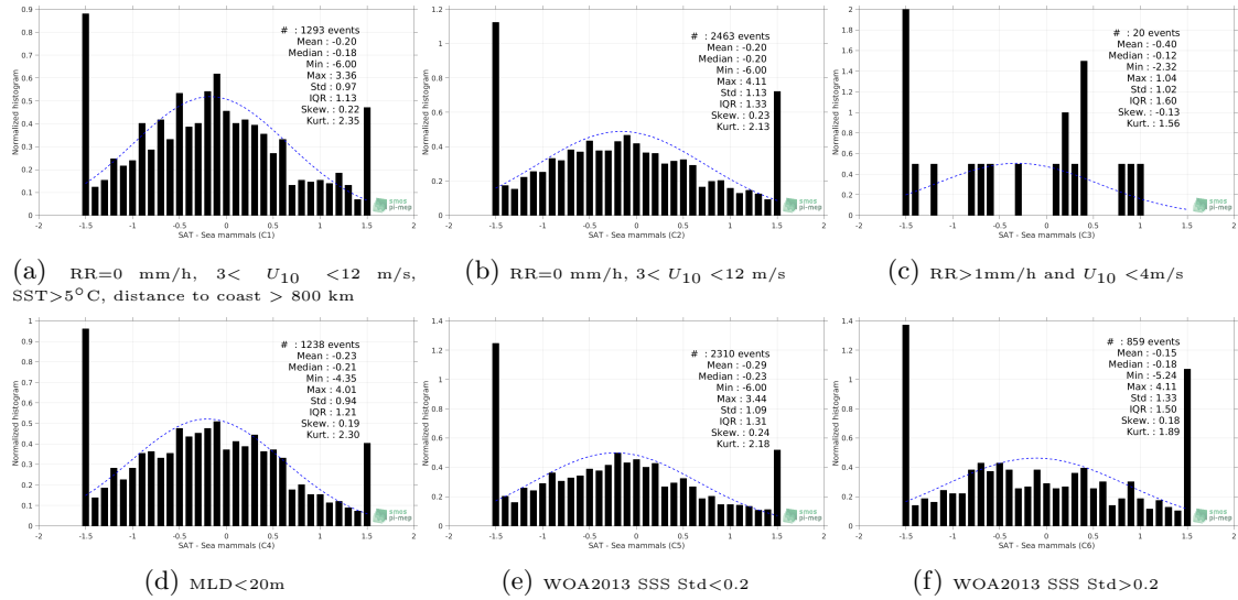
Figure 13: Normalized histogram of \Delta SSS (SMOS SSS L2 v700 (ESA) - Sea mammals) for 6 different subdatasets corresponding to: RR=0 mm/h, 3 < U_{10} < 12 m/s, SST>5°C, distance to coast > 800 km (a), RR=0 mm/h, 3 < U_{10} < 12 m/s (b), RR>1mm/h and U_{10} < 4 m/s (c), MLD<20m (d), WOA2013 SSS Std<0.2 (e), WOA2013 SSS Std>0.2 (f).
