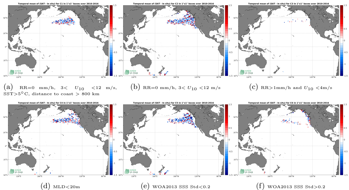
Figure 12: Temporal mean gridded over spatial boxes of size 1^\circ \times 1^\circ of \Delta SSS (SMOS SSS L2 v700 (ESA) - Sea mammals) for 6 different subdatasets corresponding to:RR=0 mm/h, 3 < U_{10} < 12 m/s, SST > 5°C, distance to coast > 800 km (a), RR=0 mm/h, 3 < U_{10} < 12 m/s (b), RR > 1mm/h and U_{10} < 4 m/s (c),MLD < 20m (d),WOA2013 SSS Std < 0.2 (e),WOA2013 SSS Std > 0.2 (f).
