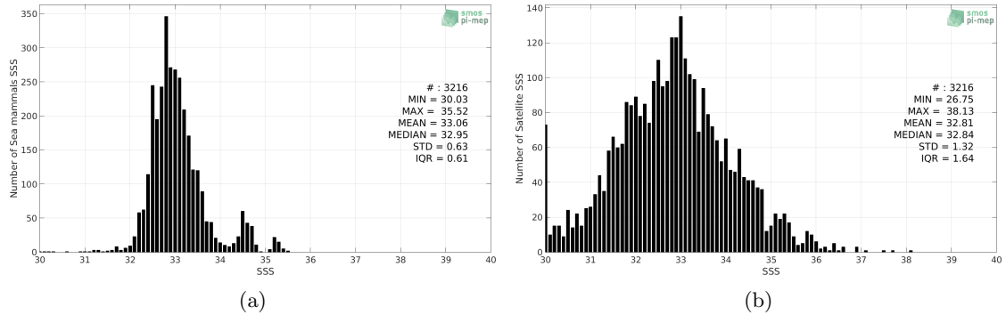
Figure 2: Histograms of SSS from Sea mammals (a) and SMOS SSS L2 v700 (ESA) (b) considering all match-up pairs per bins of 0.1 over the Pacific Ocean Pi-MEP region and for the full satellite product period.
