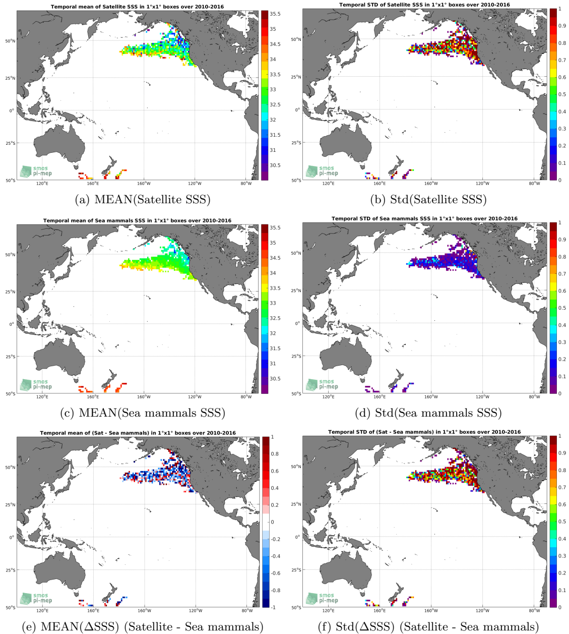
Figure 6: Temporal mean (left) and Std (right) of SSS from SMOS SSS L2 v700 (ESA) (top), Sea mammals (middle), and of \Delta SSS (Satellite - Sea mammals). Only match-up pairs are used to generate these maps.
