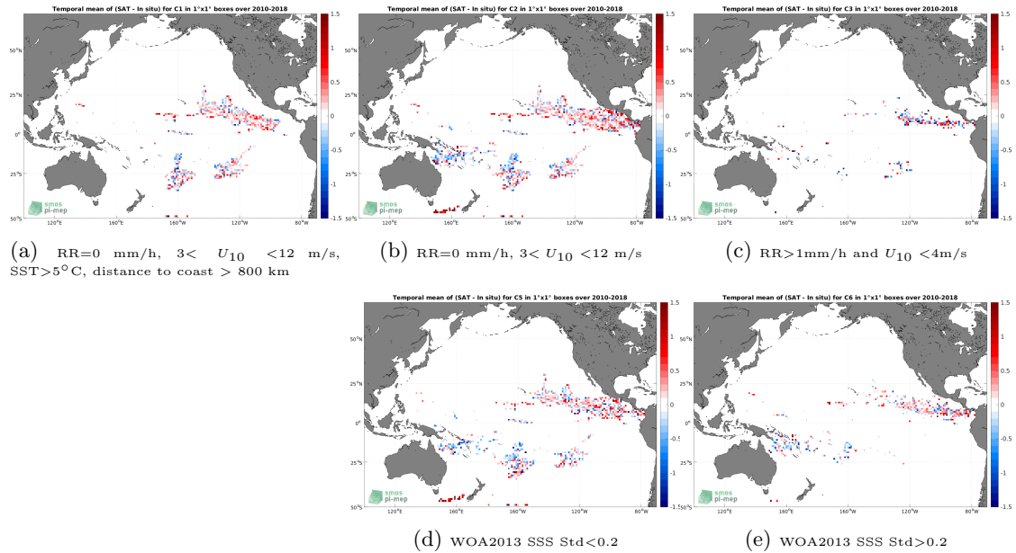
Figure 11: Temporal mean gridded over spatial boxes of size 1^\circ \times 1^\circ of \Delta\text{SSS} (SMOS SSS L2 v700 (ESA) - Surface drifters) for 5 different subdatasets corresponding to:RR=0 mm/h, 3 < U_{10} < 12 m/s, SST >5^\circ\text{C} , distance to coast > 800 km (a), RR=0 mm/h, 3 < U_{10} < 12 m/s (b), RR >1 mm/h and U_{10} < 4 m/s (c), WOA2013 SSS Std <0.2 (d), WOA2013 SSS Std >0.2 (e).
