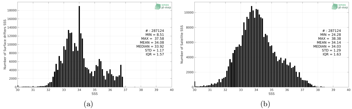
Figure 2: Histograms of SSS from Surface drifters (a) and SMOS SSS L2 v700 (ESA) (b) considering all match-up pairs per bins of 0.1 over the Pacific Ocean Pi-MEP region and for the full satellite product period.
