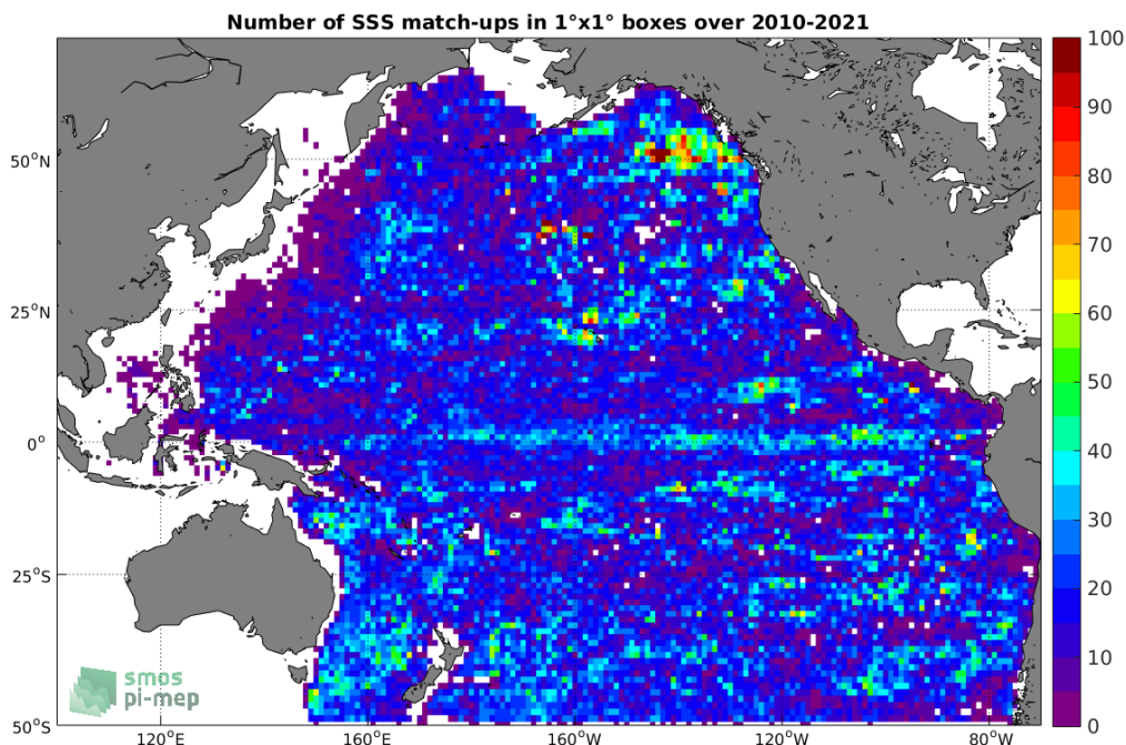
Figure 4: Number of SSS match-ups between Argo SSS and the SMOS SSS L2 v700 (ESA) SSS product for the Pacific Ocean Pi-MEP region over 1°x1° boxes and for the full satellite product period.
