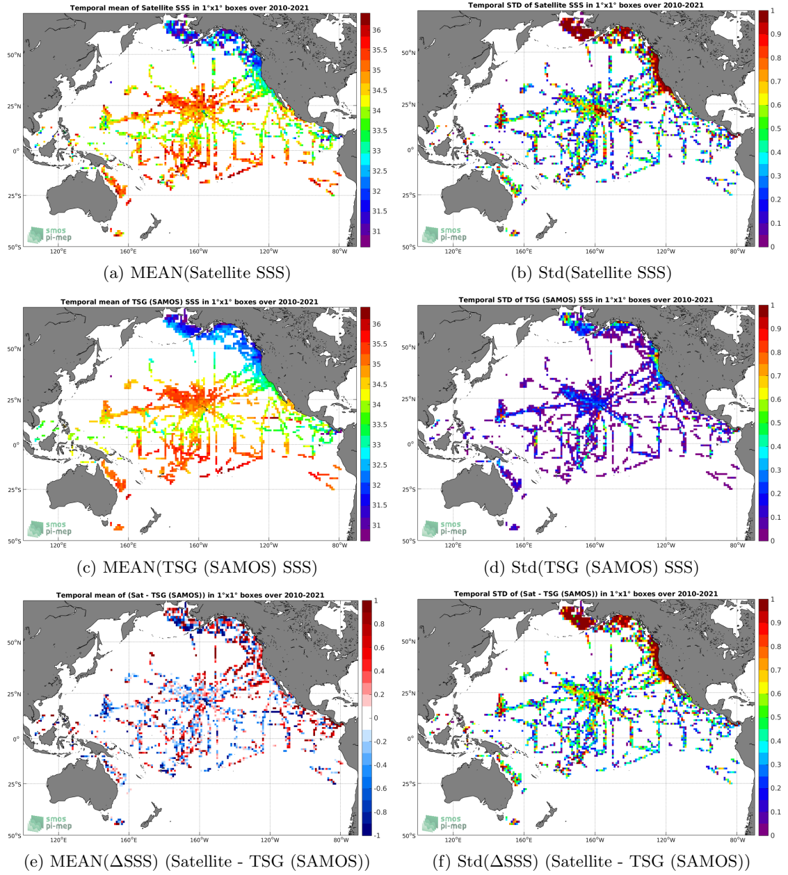
Figure 6: Temporal mean (left) and Std (right) of SSS from SMOS SSS L2 v662 (ESA) (top), TSG (SAMOS) (middle), and of \Delta SSS (Satellite - TSG (SAMOS)). Only match-up pairs are used to generate these maps.
