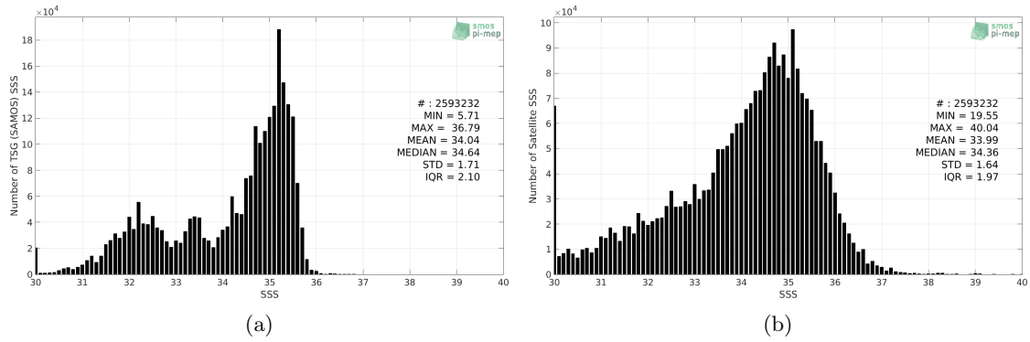
Figure 2: Histograms of SSS from TSG (SAMOS) (a) and SMOS SSS L2 v662 (ESA) (b) considering all match-up pairs per bins of 0.1 over the Pacific Ocean Pi-MEP region and for the full satellite product period.
