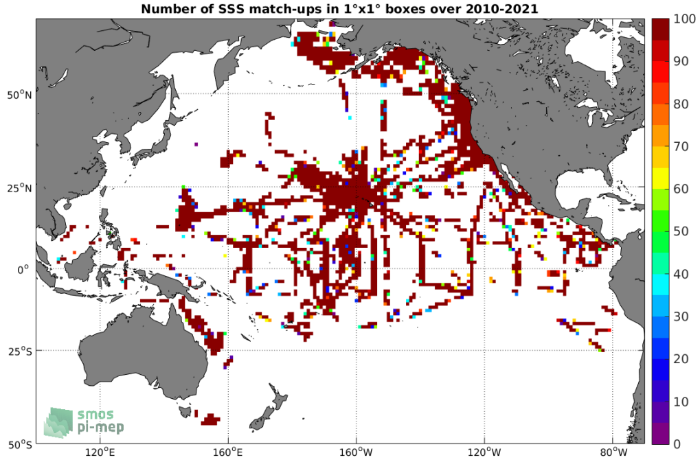
Figure 4: Number of SSS match-ups between TSG (SAMOS) SSS and the SMOS SSS L2 v662 (ESA) SSS product for the Pacific Ocean Pi-MEP region over 1^\circ \times 1^\circ boxes and for the full satellite product period.
