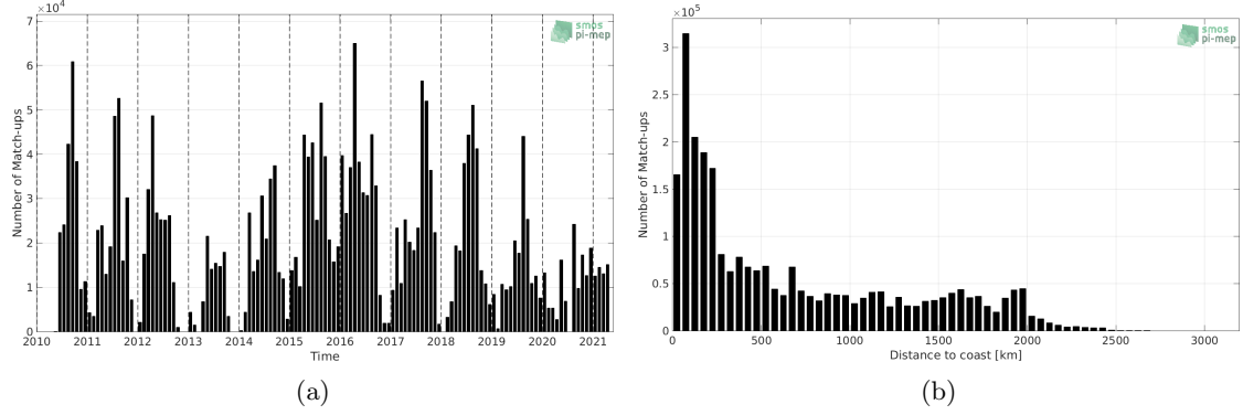
Figure 1: Number of match-ups between TSG (SAMOS) and SMOS SSS L2 v662 (ESA) SSS as a function of time (a) and as function of the distance to coast (b) over the Pacific Ocean Pi-MEP region and for the full satellite product period.
