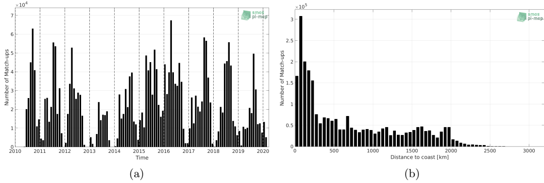
Figure 1: Number of match-ups between TSG-SAMOS and SMOS L2 v662 (ESA) SSS as a function of time (a) and as function of the distance to coast (b) over the Pacific Ocean Pi-MEP region and for the full satellite product period.
