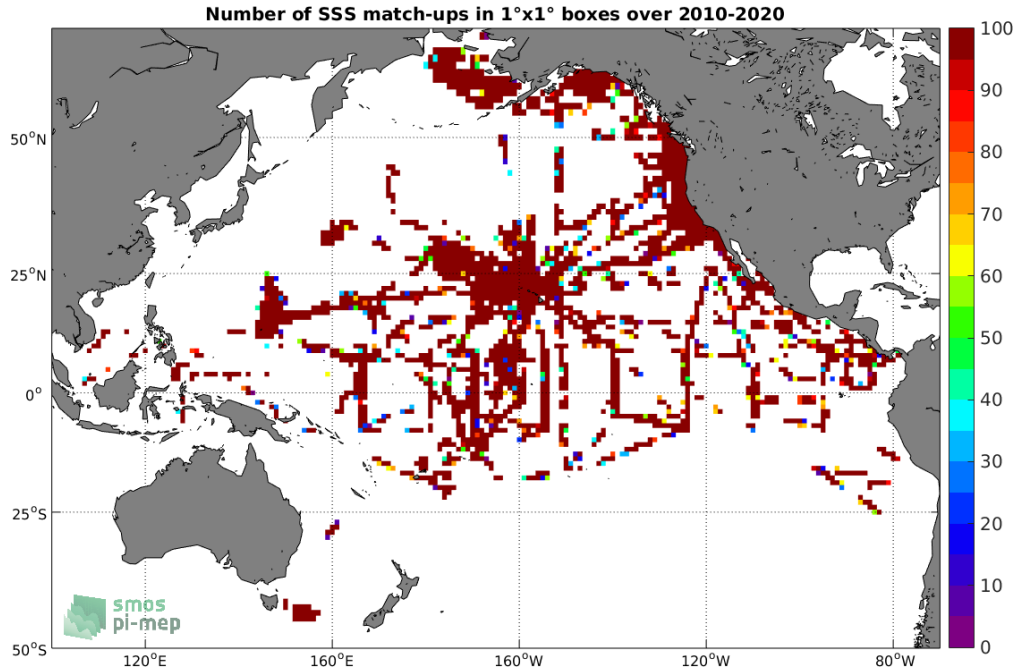
Figure 4: Number of SSS match-ups between TSG-SAMOS SSS and the SMOS L2 v662 (ESA) SSS product for the Pacific Ocean Pi-MEP region over 1°x1° boxes and for the full satellite product period.
