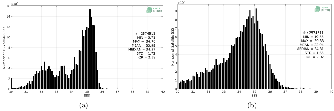
Figure 2: Histograms of SSS from TSG-SAMOS (a) and SMOS L2 v662 (ESA) (b) considering all match-up pairs per bins of 0.1 over the Pacific Ocean Pi-MEP region and for the full satellite product period.
