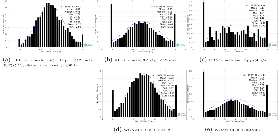
Figure 13: Normalized histogram of \Delta SSS (SMOS L2 v662 (ESA) - TSG-SAMOS) for 5 different subdatasets corresponding to: RR=0 mm/h, 3 < U_{10} < 12 m/s, SST > 5°C, distance to coast > 800 km (a), RR=0 mm/h, 3 < U_{10} < 12 m/s (b), RR > 1mm/h and U_{10} < 4 m/s (c), WOA2013 SSS Std < 0.2 (d), WOA2013 SSS Std > 0.2 (e).
