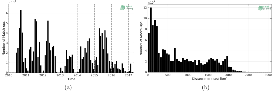
Figure 1: Number of match-ups between TSG-SAMOS and SMOS-L2-DPGS-v662 SSS as a function of time (a) and as function of the distance to coast (b) over the Pacific Ocean Pi-MEP region and for the full satellite product period.
