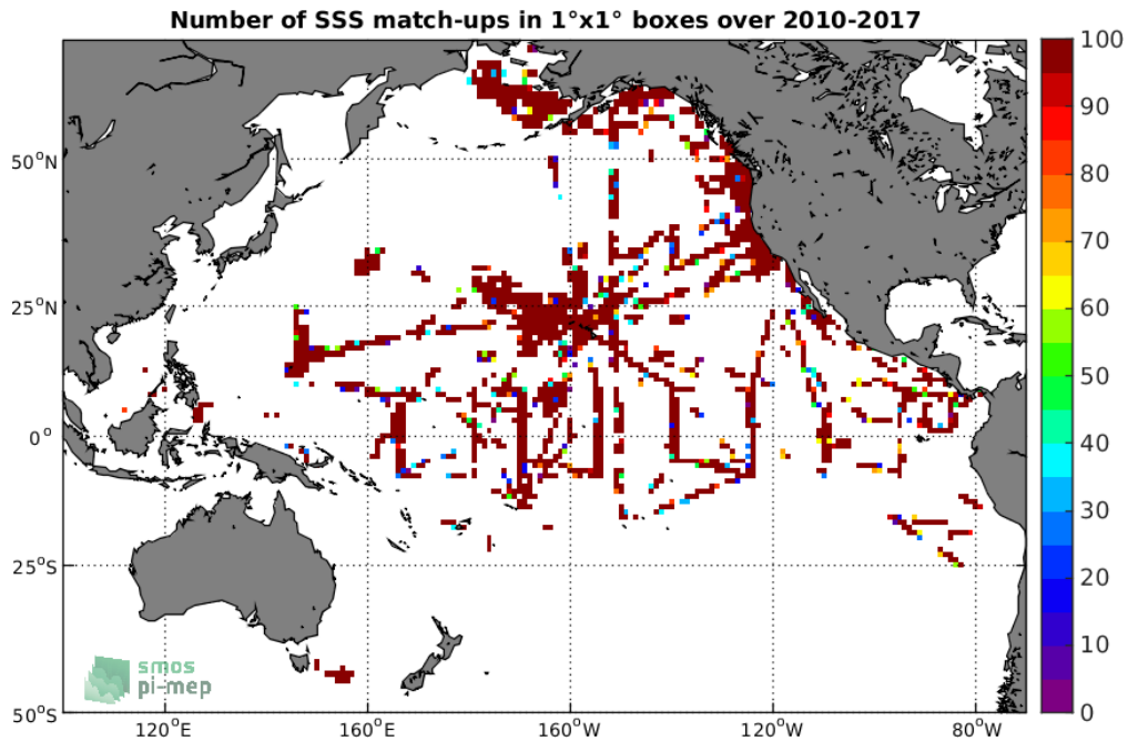
Figure 4: Number of SSS match-ups between TSG-SAMOS SSS and the SMOS-L2-DPGS-v662 SSS product for the Pacific Ocean Pi-MEP region over 1°x1° boxes and for the full satellite product period.
