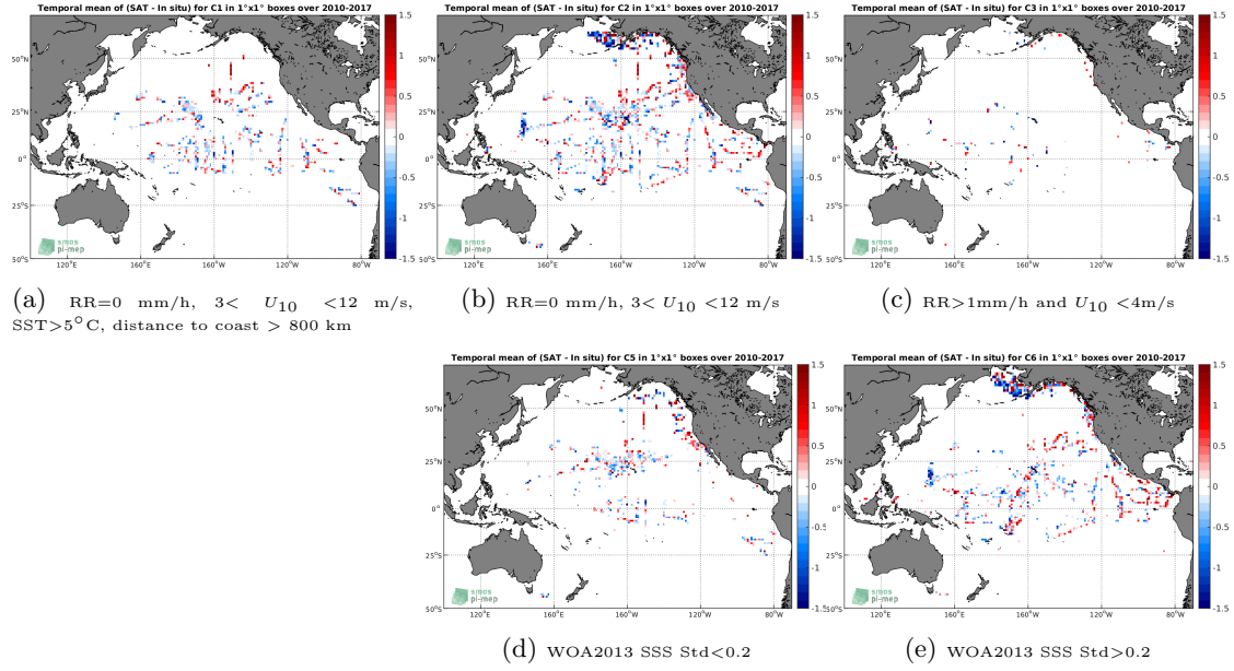
Figure 12: Temporal mean gridded over spatial boxes of size 1^\circ \times 1^\circ of \Delta SSS (SMOS-L2-DPGS-v662 - TSG-SAMOS) for 5 different subdatasets corresponding to: RR=0 mm/h, 3 < U_{10} < 12 m/s, SST >5^\circ\text{C} , distance to coast > 800 km (a), RR=0 mm/h, 3 < U_{10} < 12 m/s (b), RR >1 mm/h and U_{10} < 4 m/s (c), WOA2013 SSS Std <0.2 (d), WOA2013 SSS Std >0.2 (e).
