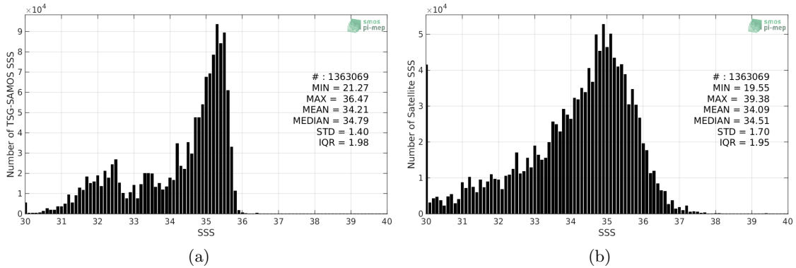
Figure 2: Histograms of SSS from TSG-SAMOS (a) and SMOS-L2-DPGS-v662 (b) considering all match-up pairs per bins of 0.1 over the Pacific Ocean Pi-MEP region and for the full satellite product period.
