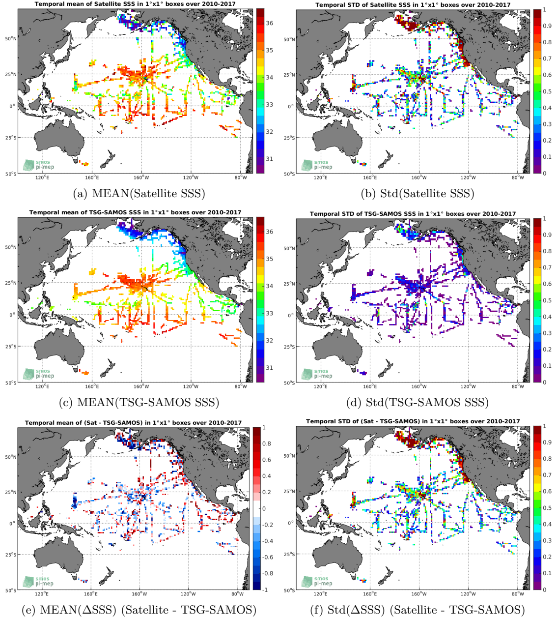
Figure 6: Temporal mean (left) and Std (right) of SSS from SMOS-L2-DPGS-v662 (top), TSG-SAMOS (middle), and of \Delta SSS (Satellite - TSG-SAMOS). Only match-up pairs are used to generate these maps.
