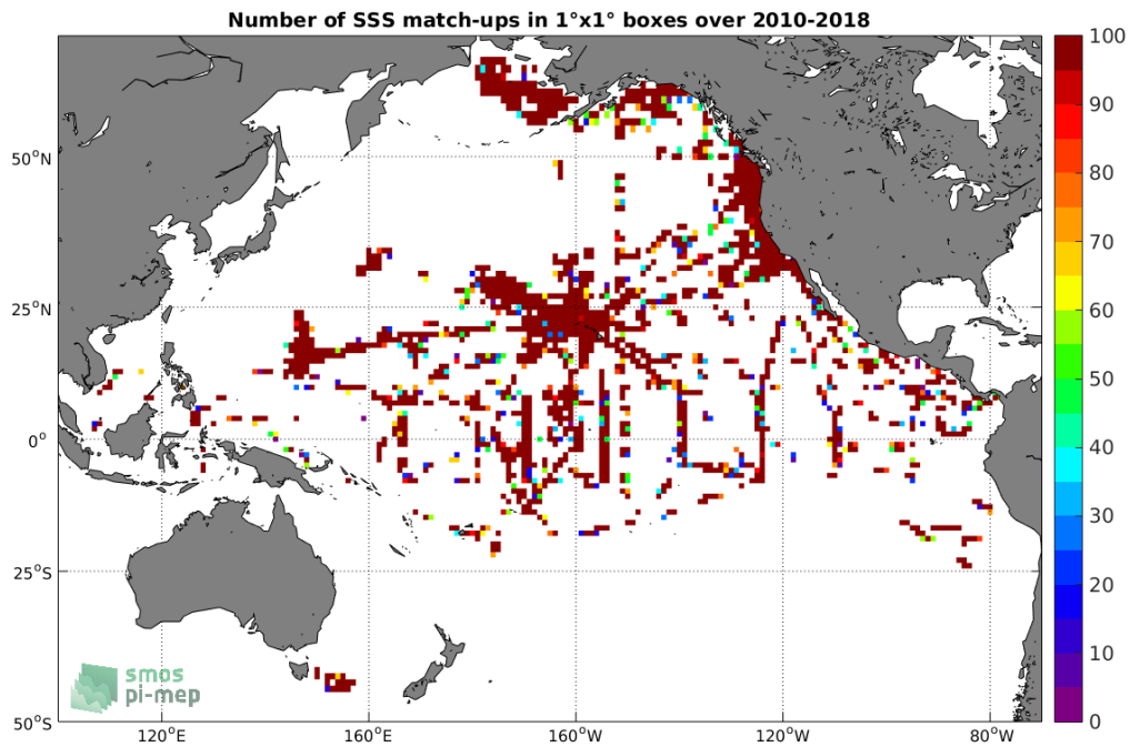
Figure 4: Number of SSS match-ups between TSG-SAMOS SSS and the SMOS-L2-DPGS-v662 SSS product for the Pacific Ocean Pi-MEP region over 1^\circ \times 1^\circ boxes and for the full satellite product period.
