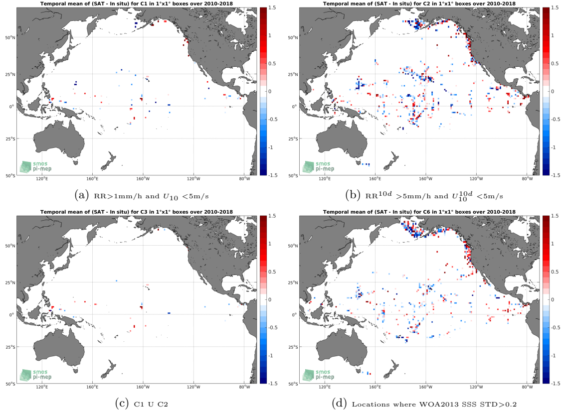
Figure 12: Temporal mean gridded over spatial boxes of size 1^\circ \times 1^\circ of \Delta SSS (SMOS-L2-DPGS-v662 - TSG-SAMOS) for 4 different subdatasets corresponding to: RR > 1mm/h and U_{10} < 5\text{m/s} (a), RR^{10d} > 5\text{mm/h} and U_{10}^{10d} < 5\text{m/s} (b), C1 U C2 (c), Locations where WOA2013 SSS STD > 0.2 (d).
