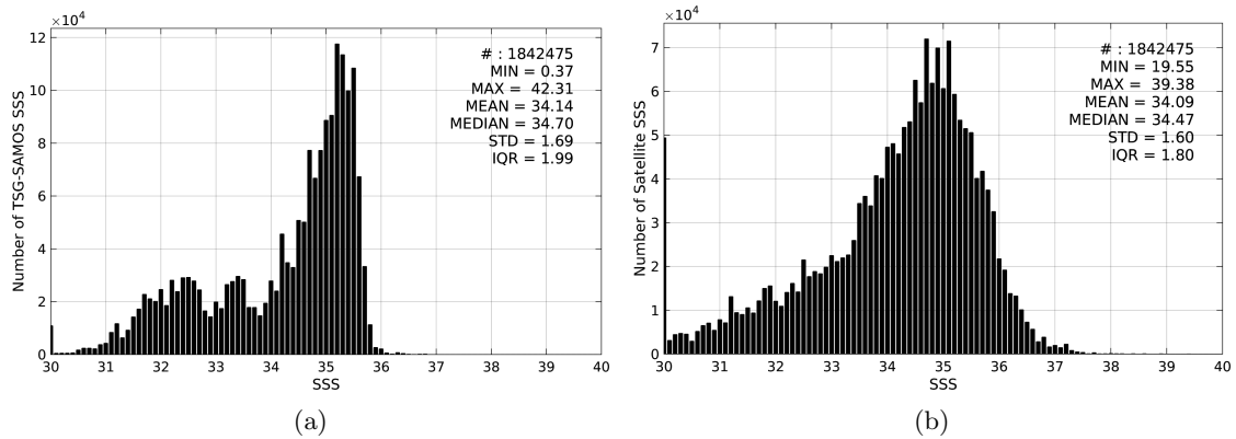
Figure 2: Histograms of SSS from TSG-SAMOS (a) and SMOS-L2-DPGS-v662 (b) considering all match-up pairs per bins of 0.1 over the Pacific Ocean Pi-MEP region and for the full satellite product period.
