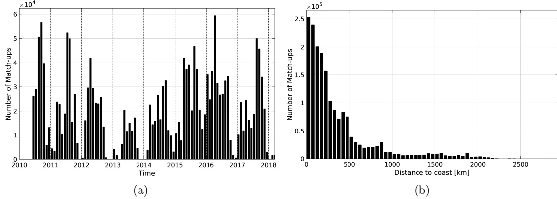
Figure 1: Number of match-ups between TSG-SAMOS and SMOS-L2-DPGS-v662 SSS as a function of time (a) and as function of the distance to coast (b) over the Pacific Ocean Pi-MEP region and for the full satellite product period.
