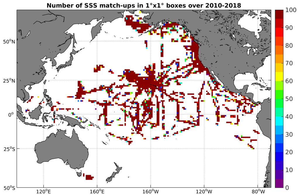
Figure 4: Number of SSS match-ups between TSG-SAMOS SSS and the SMOS-L2-DPGS-v662 SSS product for the Pacific Ocean Pi-MEP region over 1^\circ \times 1^\circ boxes and for the full satellite product period.
