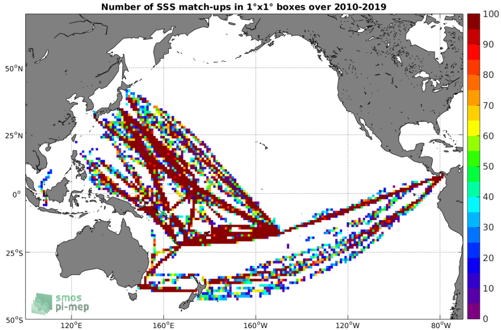
Figure 4: Number of SSS match-ups between TSG-LEGOS-DM SSS and the SMOS L2 v662 (ESA) SSS product for the Pacific Ocean Pi-MEP region over 1^\circ \times 1^\circ boxes and for the full satellite product period.
