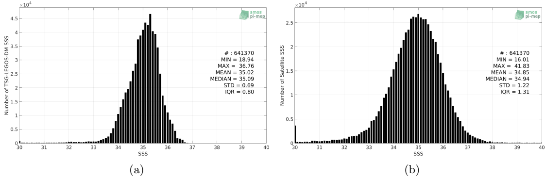
Figure 2: Histograms of SSS from TSG-LEGOS-DM (a) and SMOS L2 v662 (ESA) (b) considering all match-up pairs per bins of 0.1 over the Pacific Ocean Pi-MEP region and for the full satellite product period.
