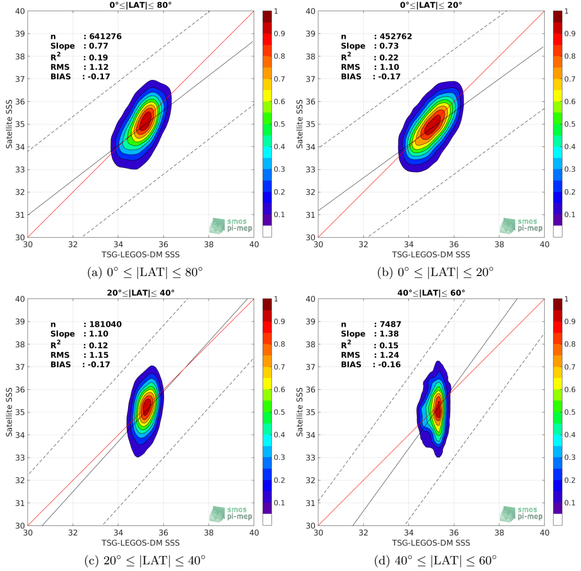
Figure 9: Contour maps of the concentration of SMOS L2 v662 (ESA) SSS (y-axis) versus TSG-LEGOS-DM SSS (x-axis) at match-up pairs for different latitude bands. For each plot, the red line shows x=y . The black thin and dashed lines indicate a linear fit through the data cloud and the \pm 95\% confidence levels, respectively. The number match-up pairs n , the slope and R^2 coefficient of the linear fit, the root mean square (RMS) and the mean bias between satellite and in situ data are indicated for each latitude band in each plots.
