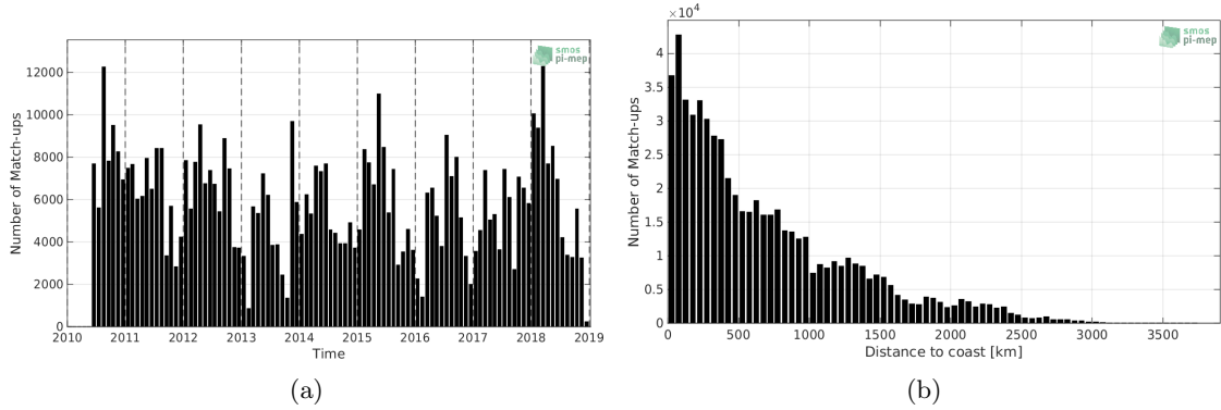
Figure 1: Number of match-ups between TSG-LEGOS-DM and SMOS-L2-DPGS-v662 SSS as a function of time (a) and as function of the distance to coast (b) over the Pacific Ocean Pi-MEP region and for the full satellite product period.
