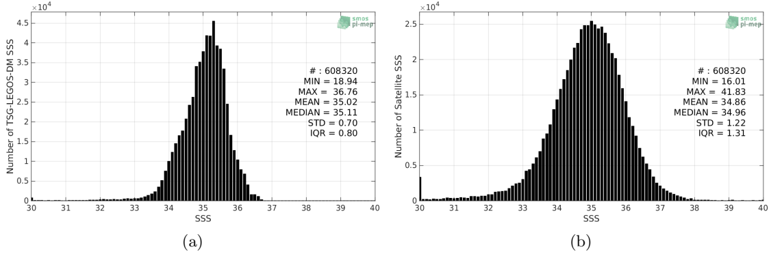
Figure 2: Histograms of SSS from TSG-LEGOS-DM (a) and SMOS-L2-DPGS-v662 (b) considering all match-up pairs per bins of 0.1 over the Pacific Ocean Pi-MEP region and for the full satellite product period.
