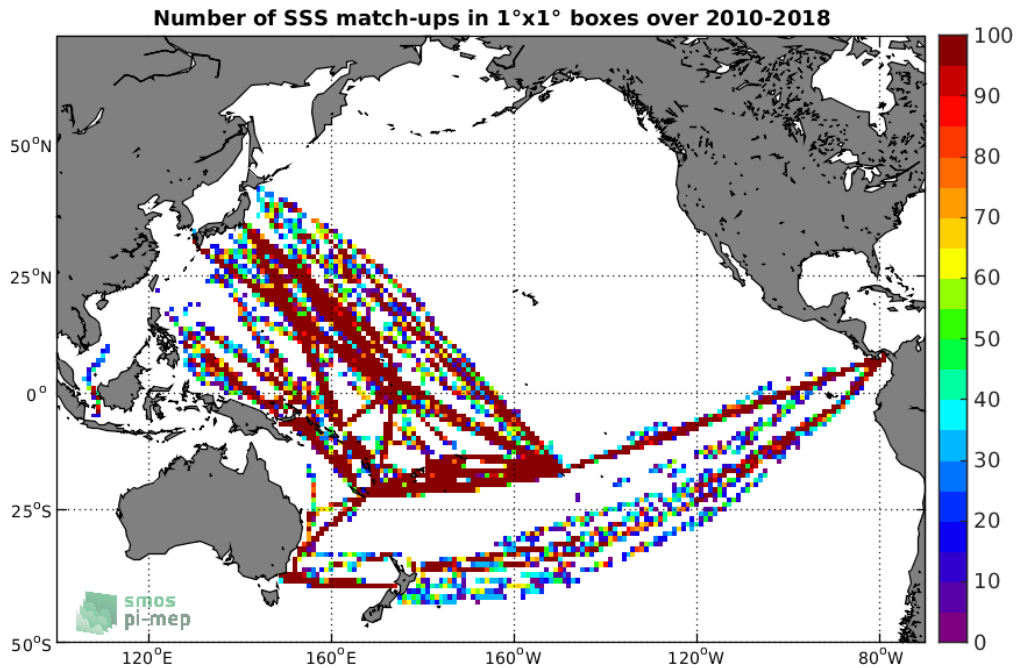
Figure 4: Number of SSS match-ups between TSG-LEGOS-DM SSS and the SMOS-L2-DPGS-v662 SSS product for the Pacific Ocean Pi-MEP region over 1^\circ \times 1^\circ boxes and for the full satellite product period.
