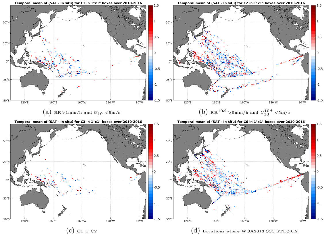
Figure 12: Temporal mean gridded over spatial boxes of size 1^\circ \times 1^\circ of \Delta SSS (SMOS-L2-DPGS-v662 - TSG-LEGOS-DM) for 4 different subdatasets corresponding to: RR > 1 mm/h and U_{10} < 5 m/s (a), RR 10d > 5 mm/h and U_{10}^{10d} < 5 m/s (b), C1 U C2 (c), Locations where WOA2013 SSS STD > 0.2 (d).
