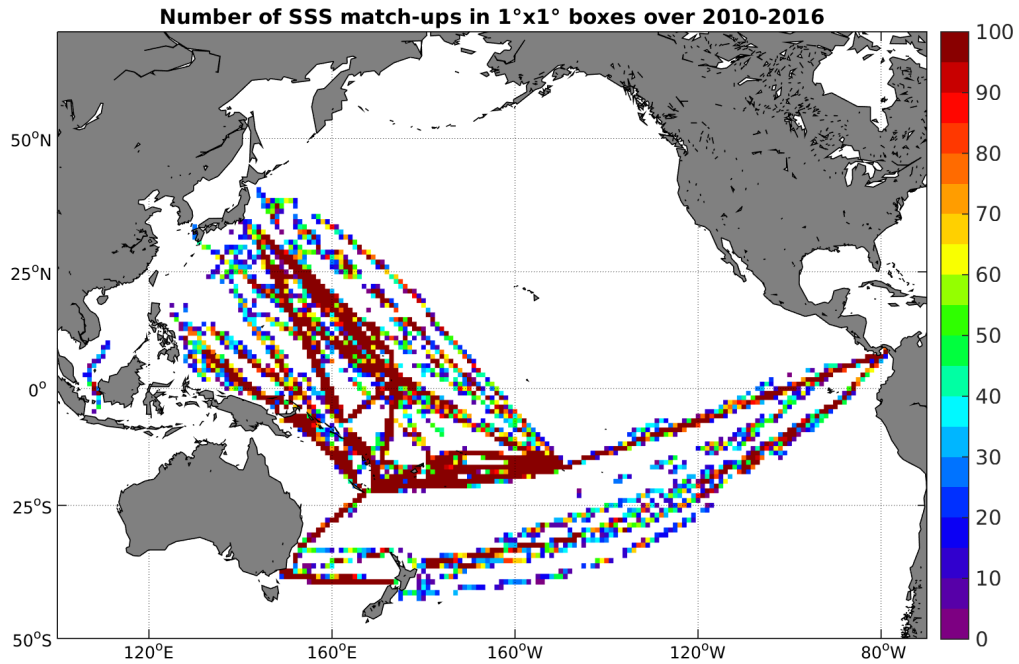
Figure 4: Number of SSS match-ups between TSG-LEGOS-DM SSS and the SMOS-L2-DPGS-v662 SSS product for the Pacific Ocean Pi-MEP region over 1^\circ \times 1^\circ boxes and for the full satellite product period.
