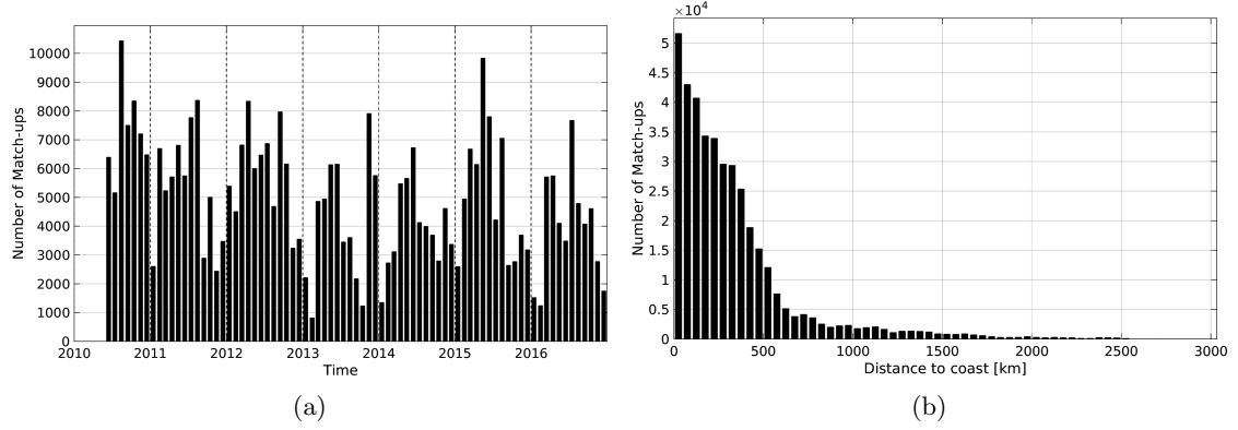
Figure 1: Number of match-ups between TSG-LEGOS-DM and SMOS-L2-DPGS-v662 SSS as a function of time (a) and as function of the distance to coast (b) over the Pacific Ocean Pi-MEP region and for the full satellite product period.
