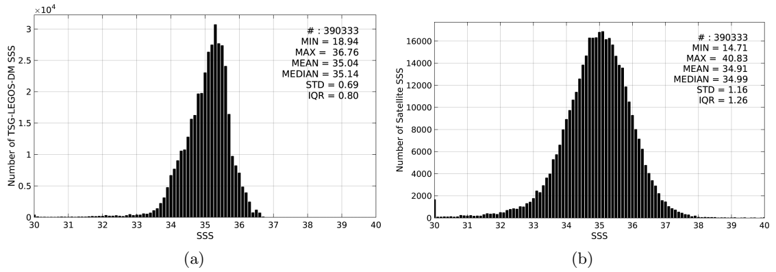
Figure 2: Histograms of SSS from TSG-LEGOS-DM (a) and SMOS-L2-DPGS-v662 (b) considering all match-up pairs per bins of 0.1 over the Pacific Ocean Pi-MEP region and for the full satellite product period.
