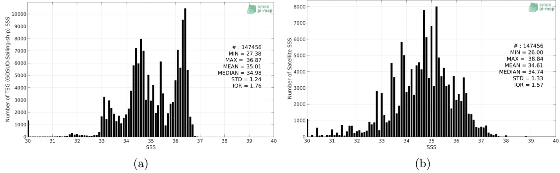
Figure 2: Histograms of SSS from TSG (GOSUD-Sailing-ship) (a) and SMOS SSS L2 v662 (ESA) (b) considering all match-up pairs per bins of 0.1 over the Pacific Ocean Pi-MEP region and for the full satellite product period.
