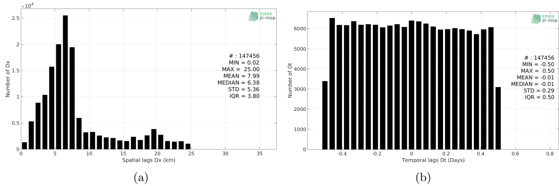
Figure 5: Histograms of the spatial (a) and temporal (b) lags between the location/time of the TSG (GOSUD-Sailing-ship) measurement and the date of the corresponding SMOS SSS L2 v662 (ESA) SSS pixel.
