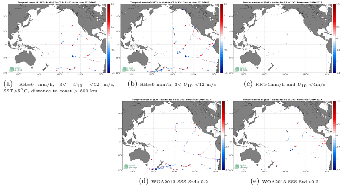
Figure 12: Temporal mean gridded over spatial boxes of size 1^\circ \times 1^\circ of \Delta SSS (SMOS SSS L2 v662 (ESA) - TSG (GOSUD-Sailing-ship)) for 5 different subdatasets corresponding to:RR=0 mm/h, 3 < U_{10} < 12 m/s, SST >5^\circ C, distance to coast > 800 km (a), RR=0 mm/h, 3 < U_{10} < 12 m/s (b), RR >1 mm/h and U_{10} < 4 m/s (c), WOA2013 SSS Std <0.2 (d), WOA2013 SSS Std >0.2 (e).
