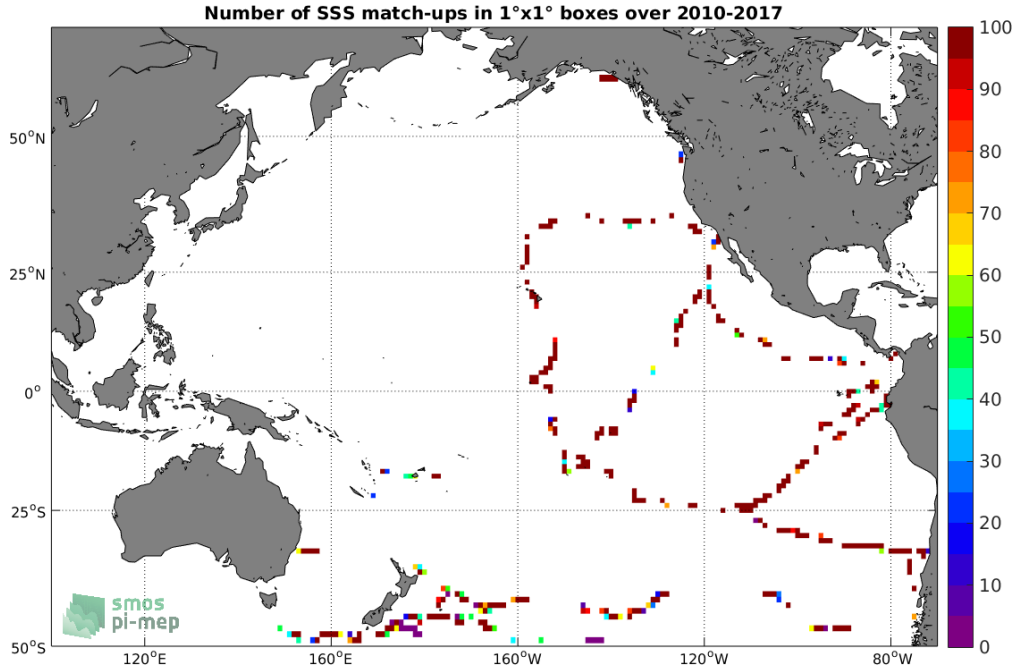
Figure 4: Number of SSS match-ups between TSG (GOSUD-Sailing-ship) SSS and the SMOS SSS L2 v662 (ESA) SSS product for the Pacific Ocean Pi-MEP region over 1^\circ \times 1^\circ boxes and for the full satellite product period.
