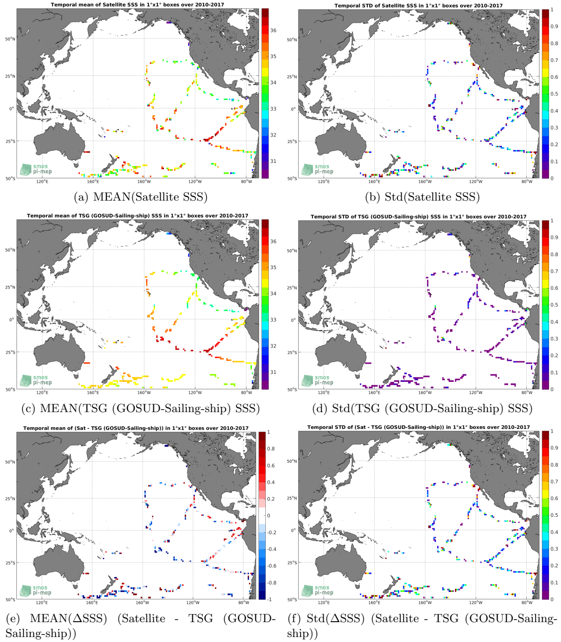
Figure 6: Temporal mean (left) and Std (right) of SSS from SMOS SSS L2 v662 (ESA) (top), TSG (GOSUD-Sailing-ship) (middle), and of \Delta SSS (Satellite - TSG (GOSUD-Sailing-ship)). Only match-up pairs are used to generate these maps.
