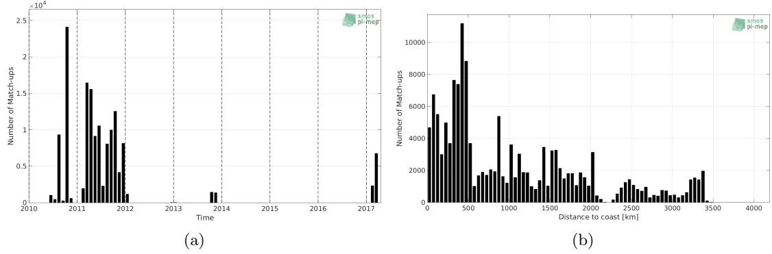
Figure 1: Number of match-ups between TSG (GOSUD-Sailing-ship) and SMOS SSS L2 v662 (ESA) SSS as a function of time (a) and as function of the distance to coast (b) over the Pacific Ocean Pi-MEP region and for the full satellite product period.
