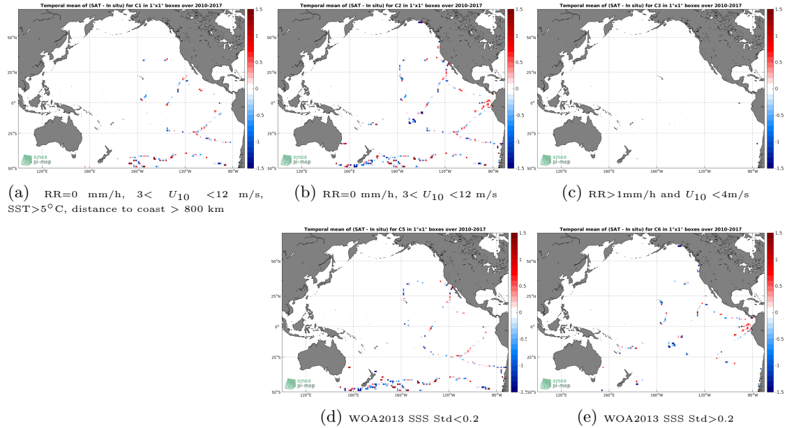
Figure 12: Temporal mean gridded over spatial boxes of size 1^\circ \times 1^\circ of \Delta SSS (SMOS SSS L2 v662 (ESA) - TSG (GOSUD-Sailing-ship)) for 5 different subdatasets corresponding to: RR=0 mm/h, 3 < U_{10} < 12 m/s, SST >5^\circ\text{C} , distance to coast > 800 km (a), RR=0 mm/h, 3 < U_{10} < 12 m/s (b), RR >1 mm/h and U_{10} < 4 m/s (c), WOA2013 SSS Std <0.2 (d), WOA2013 SSS Std >0.2 (e).
