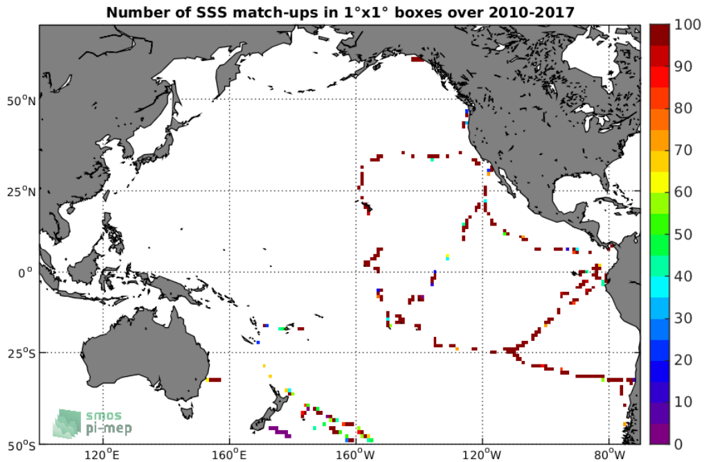
Figure 4: Number of SSS match-ups between TSG-GOSUD-Sailing-ship SSS and the SMOS-L2-DPGS-v662 SSS product for the Pacific Ocean Pi-MEP region over 1°x1° boxes and for the full satellite product period.
