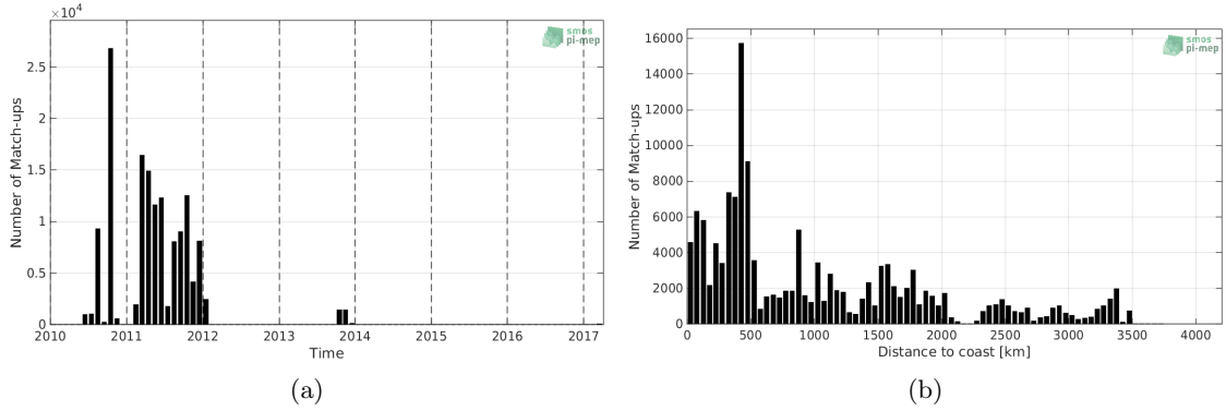
Figure 1: Number of match-ups between TSG-GOSUD-Sailing-ship and SMOS-L2-DPGS-v662 SSS as a function of time (a) and as function of the distance to coast (b) over the Pacific Ocean Pi-MEP region and for the full satellite product period.
