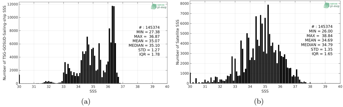
Figure 2: Histograms of SSS from TSG-GOSUD-Sailing-ship (a) and SMOS-L2-DPGS-v662 (b) considering all match-up pairs per bins of 0.1 over the Pacific Ocean Pi-MEP region and for the full satellite product period.
