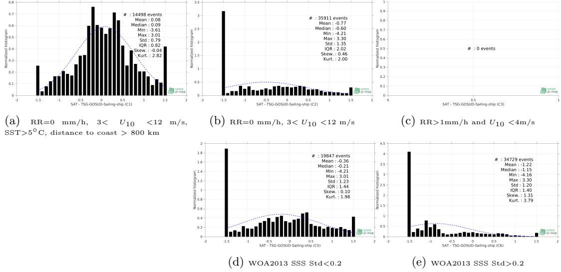
Figure 13: Normalized histogram of \Delta SSS (SMOS-L2-DPGS-v662 - TSG-GOSUD-Sailing-ship) for 5 different subdatasets corresponding to: RR=0 mm/h, 3 < U_{10} < 12 m/s, SST > 5^\circ C , distance to coast > 800 km (a), RR=0 mm/h, 3 < U_{10} < 12 m/s (b), RR > 1 mm/h and U_{10} < 4 m/s (c), WOA2013 SSS Std < 0.2 (d), WOA2013 SSS Std > 0.2 (e).
