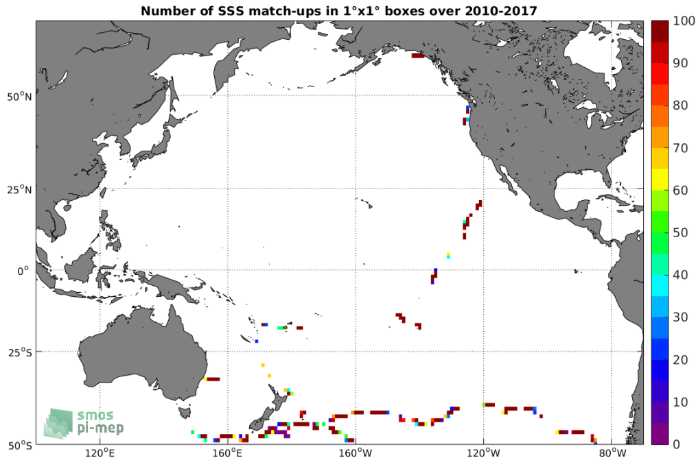
Figure 4: Number of SSS match-ups between TSG-GOSUD-Sailing-ship SSS and the SMOS-L2-DPGS-v662 SSS product for the Pacific Ocean Pi-MEP region over 1^\circ \times 1^\circ boxes and for the full satellite product period.
