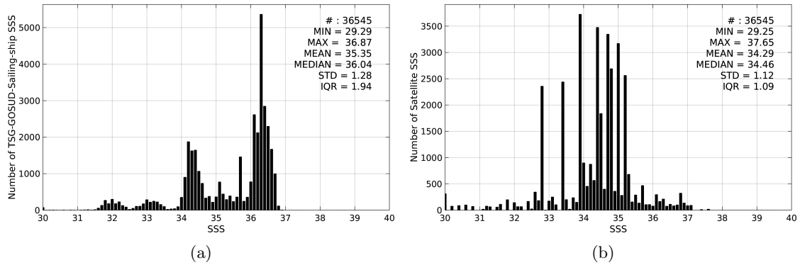
Figure 2: Histograms of SSS from TSG-GOSUD-Sailing-ship (a) and SMOS-L2-DPGS-v662 (b) considering all match-up pairs per bins of 0.1 over the Pacific Ocean Pi-MEP region and for the full satellite product period.
