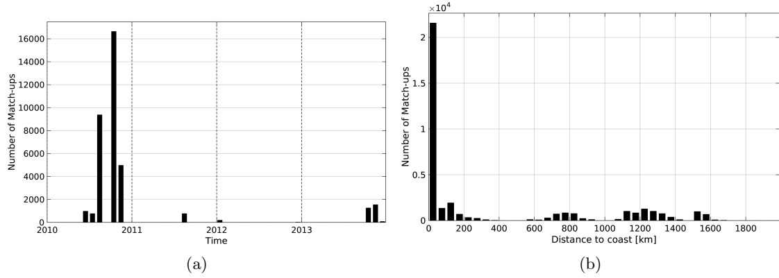
Figure 1: Number of match-ups between TSG-GOSUD-Sailing-ship and SMOS-L2-DPGS-v662 SSS as a function of time (a) and as function of the distance to coast (b) over the Pacific Ocean Pi-MEP region and for the full satellite product period.
