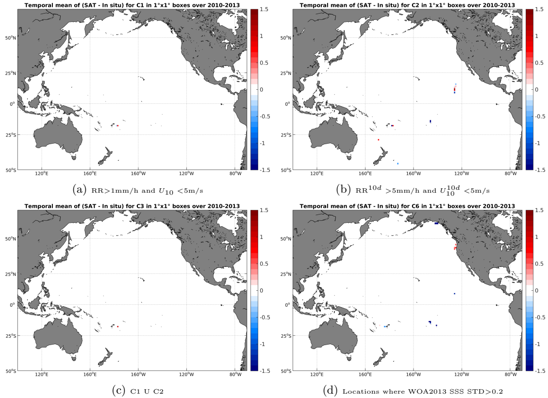
Figure 12: Temporal mean gridded over spatial boxes of size 1^\circ \times 1^\circ of \Delta SSS (SMOS-L2-DPGS-v662 - TSG-GOSUD-Sailing-ship) for 4 different subdatasets corresponding to: RR > 1\text{mm/h} and U_{10} < 5\text{m/s} (a), RR^{10d} > 5\text{mm/h} and U_{10}^{10d} < 5\text{m/s} (b), C1 U C2 (c), Locations where WOA2013 SSS STD > 0.2 (d).
