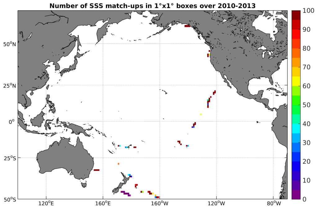
Figure 4: Number of SSS match-ups between TSG-GOSUD-Sailing-ship SSS and the SMOS-L2-DPGS-v662 SSS product for the Pacific Ocean Pi-MEP region over 1^\circ \times 1^\circ boxes and for the full satellite product period.
