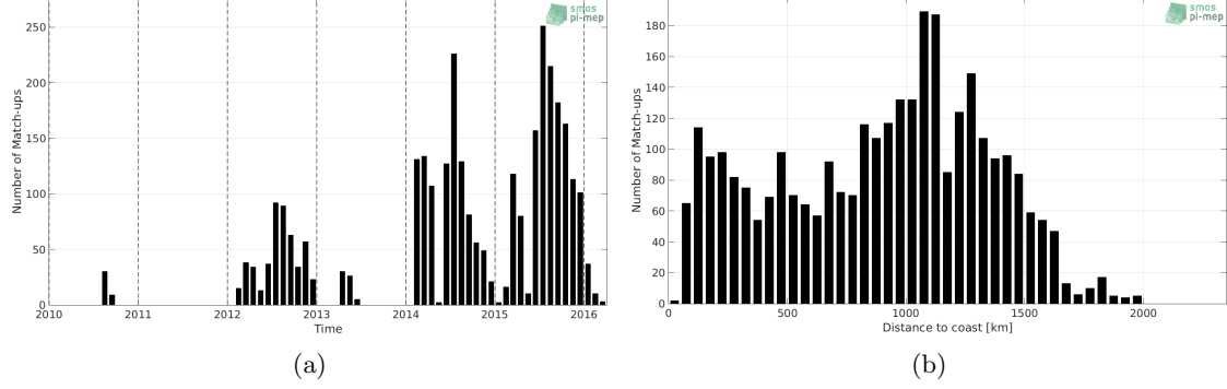
Figure 1: Number of match-ups between Sea mammals and SMOS SSS L2 v662 (ESA) SSS as a function of time (a) and as function of the distance to coast (b) over the Pacific Ocean Pi-MEP region and for the full satellite product period.
