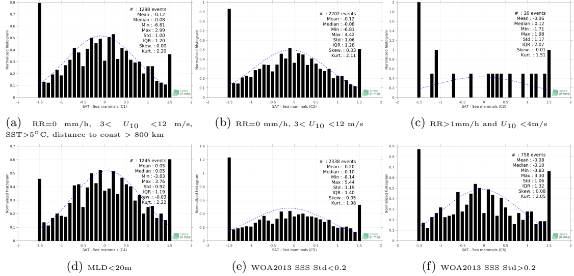
Figure 13: Normalized histogram of \Delta\text{SSS} (SMOS SSS L2 v662 (ESA) - Sea mammals) for 6 different subdatasets corresponding to: RR=0 mm/h, 3 < U_{10} < 12 m/s, SST>5°C, distance to coast > 800 km (a), RR=0 mm/h, 3 < U_{10} < 12 m/s (b), RR>1mm/h and U_{10} < 4 m/s (c), MLD<20m (d), WOA2013 SSS Std<0.2 (e), WOA2013 SSS Std>0.2 (f).
