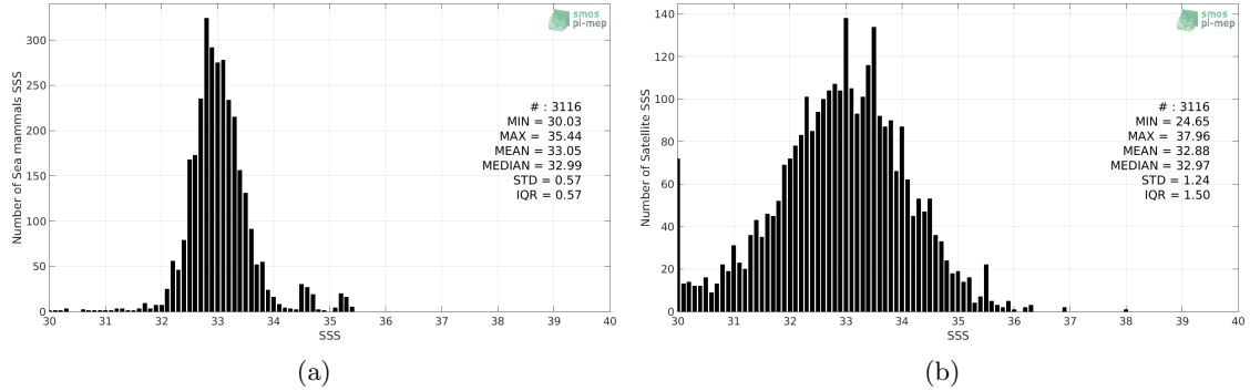
Figure 2: Histograms of SSS from Sea mammals (a) and SMOS SSS L2 v662 (ESA) (b) considering all match-up pairs per bins of 0.1 over the Pacific Ocean Pi-MEP region and for the full satellite product period.
