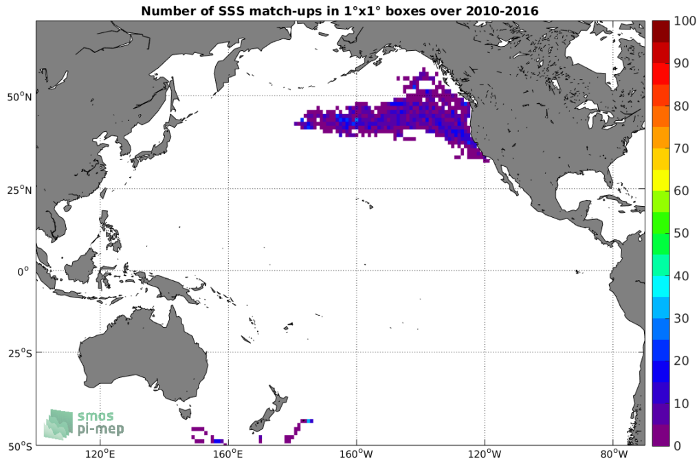
Figure 4: Number of SSS match-ups between Sea mammals SSS and the SMOS SSS L2 v662 (ESA) SSS product for the Pacific Ocean Pi-MEP region over 1°x1° boxes and for the full satellite product period.
