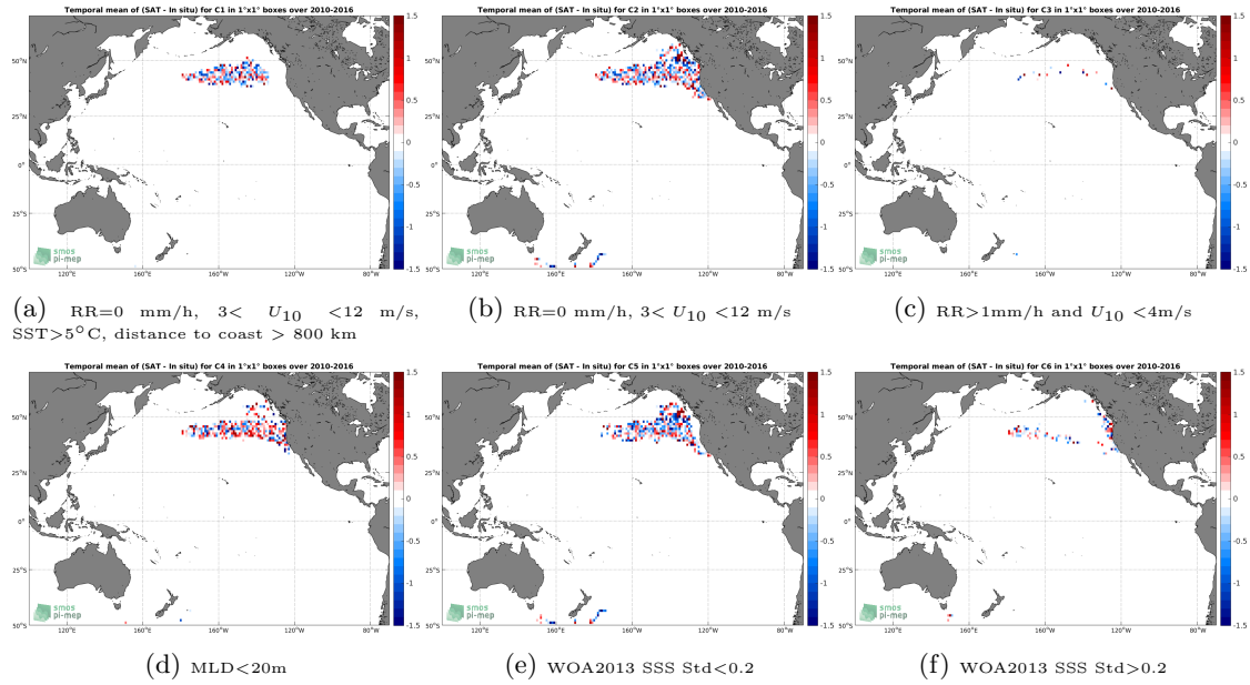
Figure 12: Temporal mean gridded over spatial boxes of size 1^\circ \times 1^\circ of \Delta SSS (SMOS SSS L2 v662 (ESA) - Sea mammals) for 6 different subdatasets corresponding to: RR=0 mm/h, 3 < U_{10} < 12 m/s, SST >5^\circ\text{C} , distance to coast > 800 km (a), RR=0 mm/h, 3 < U_{10} < 12 m/s (b), RR >1 mm/h and U_{10} < 4 m/s (c),MLD <20 m (d),WOA2013 SSS Std <0.2 (e),WOA2013 SSS Std >0.2 (f).
