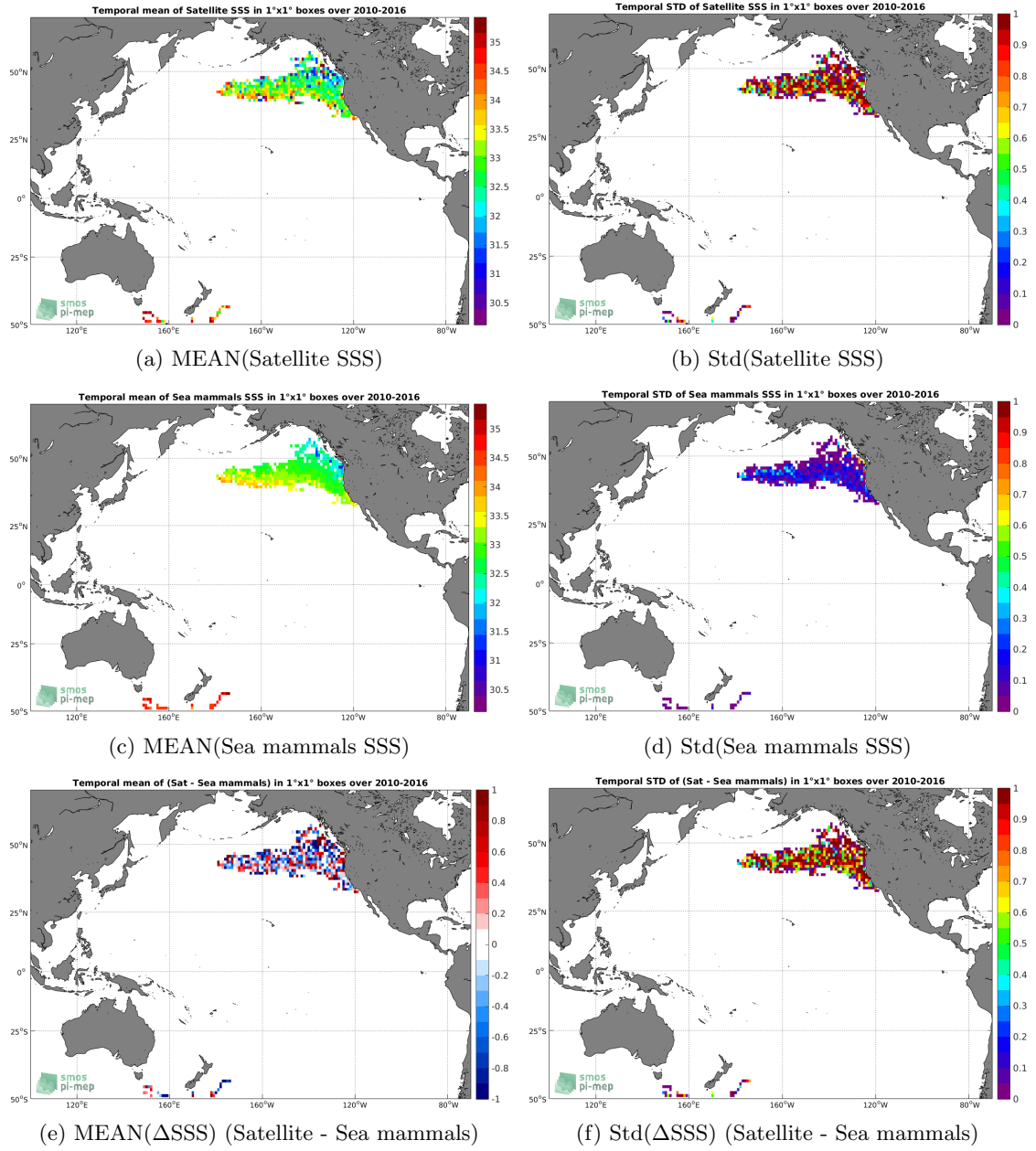
Figure 6: Temporal mean (left) and Std (right) of SSS from SMOS SSS L2 v662 (ESA) (top), Sea mammals (middle), and of ΔSSS (Satellite - Sea mammals). Only match-up pairs are used to generate these maps.
