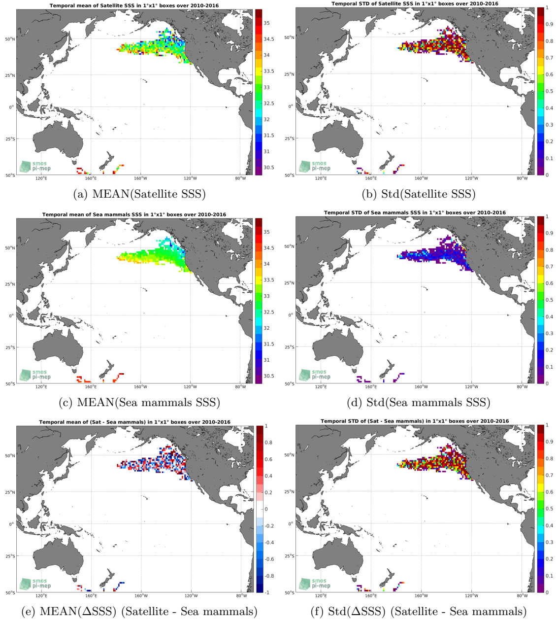
Figure 6: Temporal mean (left) and Std (right) of SSS from SMOS SSS L2 v662 (ESA) (top), Sea mammals (middle), and of \Delta SSS (Satellite - Sea mammals). Only match-up pairs are used to generate these maps.
