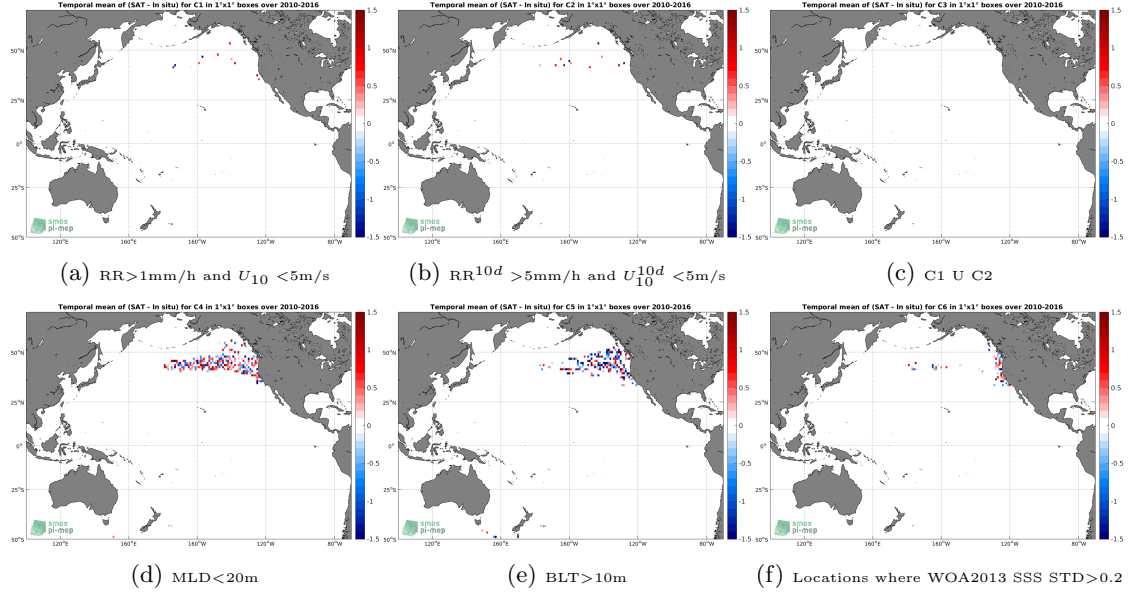
Figure 12: Temporal mean gridded over spatial boxes of size 1^\circ \times 1^\circ of \Delta\text{SSS} (SMOS-L2-DPGS-v662 - Sea mammals) for 6 different subdatasets corresponding to: RR > 1\text{mm/h} and U_{10} < 5\text{m/s} (a), RR^{10d} > 5\text{mm/h} and U_{10}^{10d} < 5\text{m/s} (b), C1 U C2 (c), MLD < 20\text{m} (d), BLT > 10\text{m} (e), Locations where WOA2013 SSS STD > 0.2 (f).
