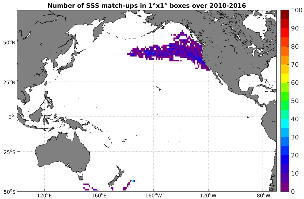
Figure 4: Number of SSS match-ups between Sea mammals SSS and the SMOS-L2-DPGS-v662 SSS product for the Pacific Ocean Pi-MEP region over 1^\circ \times 1^\circ boxes and for the full satellite product period.
