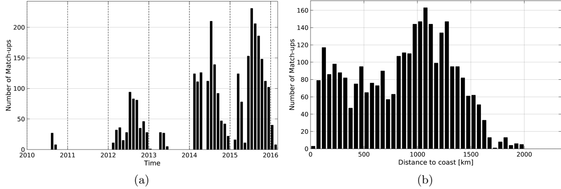
Figure 1: Number of match-ups between Sea mammals and SMOS-L2-DPGS-v662 SSS as a function of time (a) and as function of the distance to coast (b) over the Pacific Ocean Pi-MEP region and for the full satellite product period.
