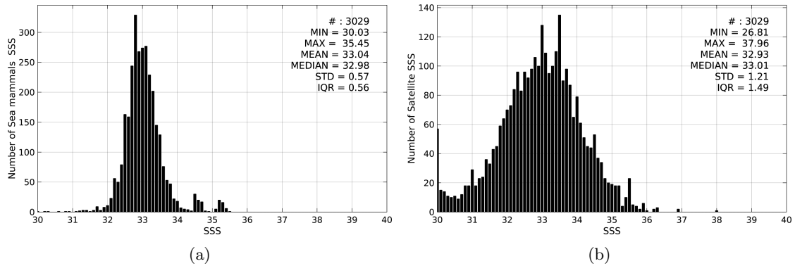
Figure 2: Histograms of SSS from Sea mammals (a) and SMOS-L2-DPGS-v662 (b) considering all match-up pairs per bins of 0.1 over the Pacific Ocean Pi-MEP region and for the full satellite product period.
