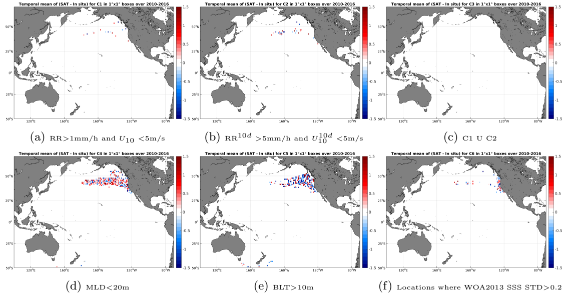
Figure 12: Temporal mean gridded over spatial boxes of size 1^\circ \times 1^\circ of \Delta SSS (SMOS-L2-DPGS-v662 - Sea mammals) for 6 different subdatasets corresponding to: RR > 1\text{mm/h} and U_{10} < 5\text{m/s} (a), RR^{10d} > 5\text{mm/h} and U_{10}^{10d} < 5\text{m/s} (b), C1 U C2 (c), MLD < 20\text{m} (d), BLT > 10\text{m} (e), Locations where WOA2013 SSS STD > 0.2 (f).
