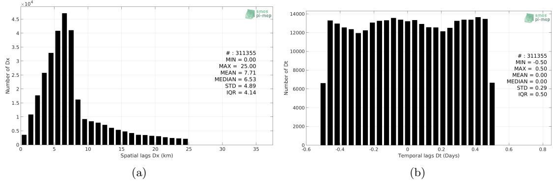
Figure 4: Histograms of the spatial (a) and temporal (b) lags between the location/time of the Surface drifters measurement and the date of the corresponding SMOS SSS L2 v662 (ESA) SSS pixel.
