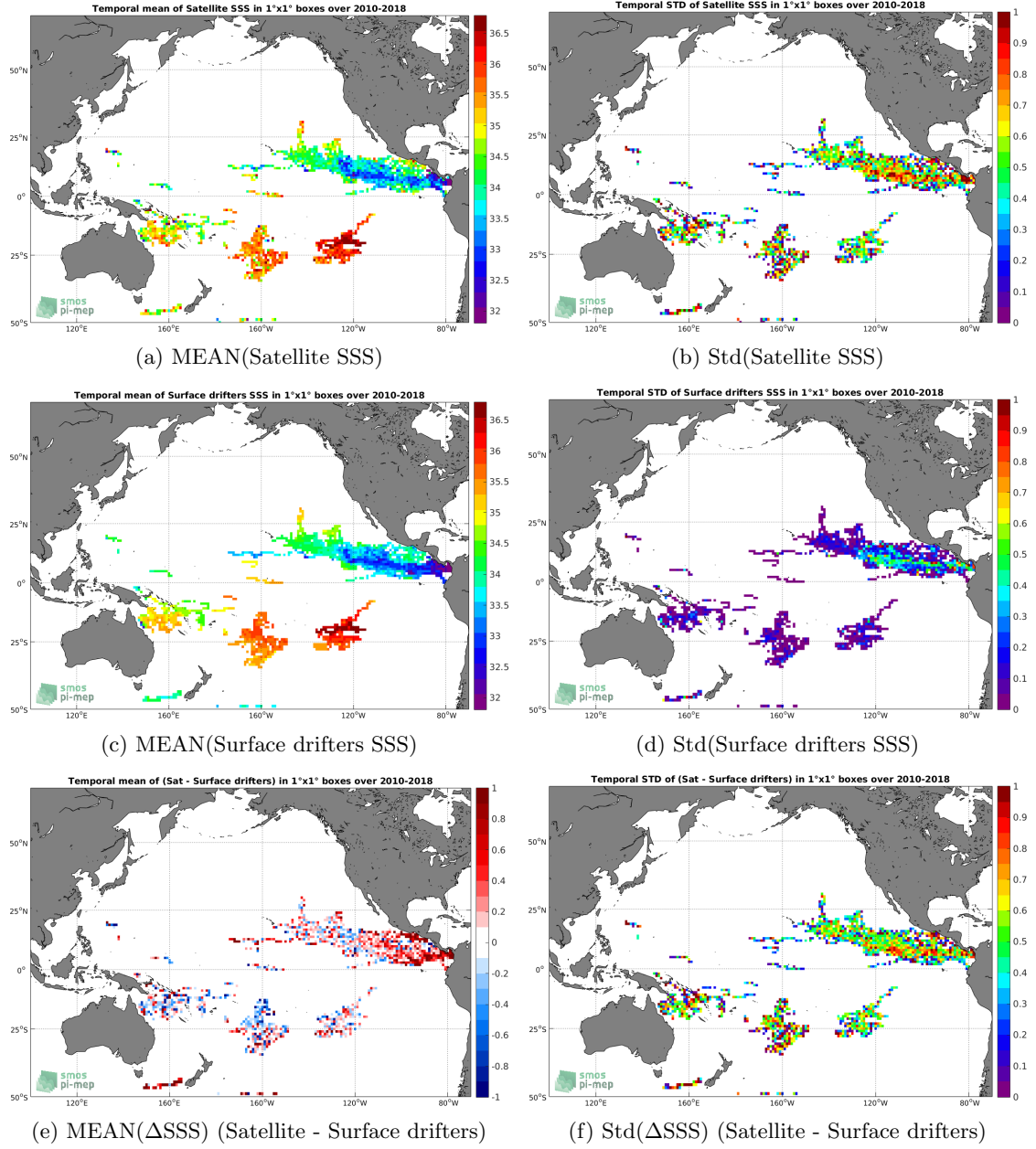
Figure 5: Temporal mean (left) and Std (right) of SSS from SMOS SSS L2 v662 (ESA) (top), Surface drifters (middle), and of \Delta SSS (Satellite - Surface drifters). Only match-up pairs are used to generate these maps.
