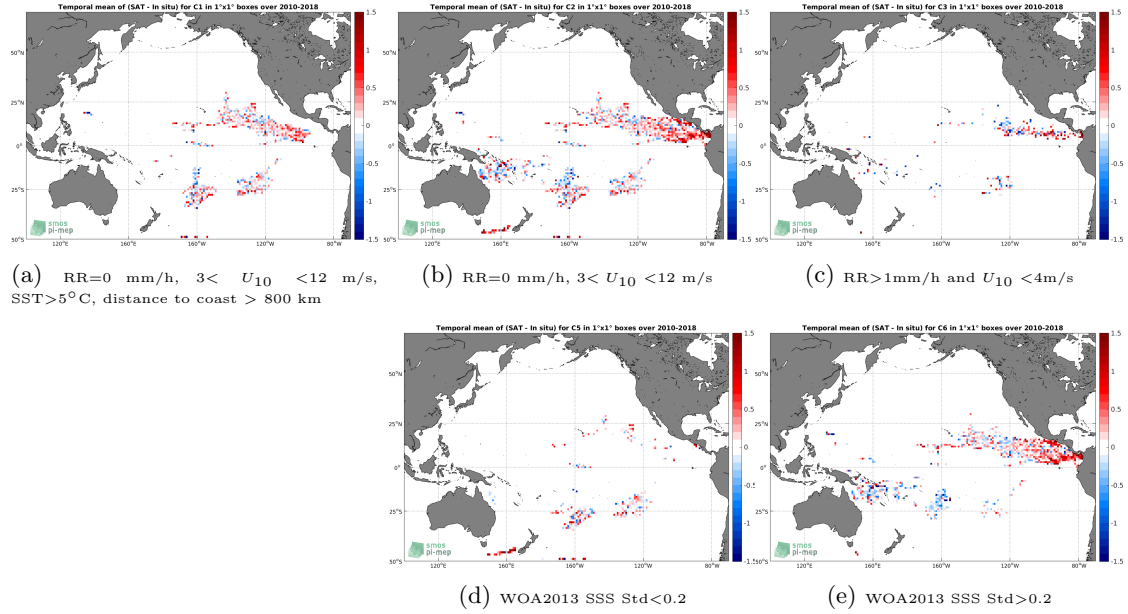
Figure 11: Temporal mean gridded over spatial boxes of size 1^\circ \times 1^\circ of \Delta SSS (SMOS SSS L2 v662 (ESA) - Surface drifters) for 5 different subdatasets corresponding to: RR=0 mm/h, 3 < U_{10} < 12 m/s, SST > 5^\circ C , distance to coast > 800 km (a), RR=0 mm/h, 3 < U_{10} < 12 m/s (b), RR > 1 mm/h and U_{10} < 4 m/s (c), WOA2013 SSS Std < 0.2 (d), WOA2013 SSS Std > 0.2 (e).
