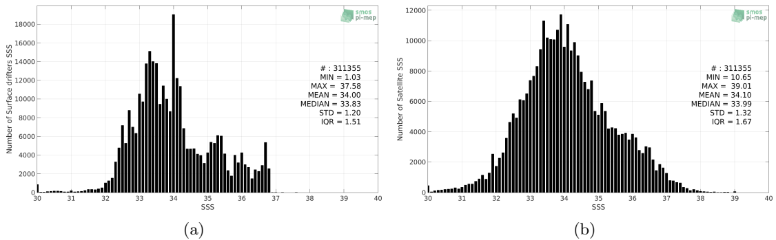
Figure 2: Histograms of SSS from Surface drifters (a) and SMOS SSS L2 v662 (ESA) (b) considering all match-up pairs per bins of 0.1 over the Pacific Ocean Pi-MEP region and for the full satellite product period.
