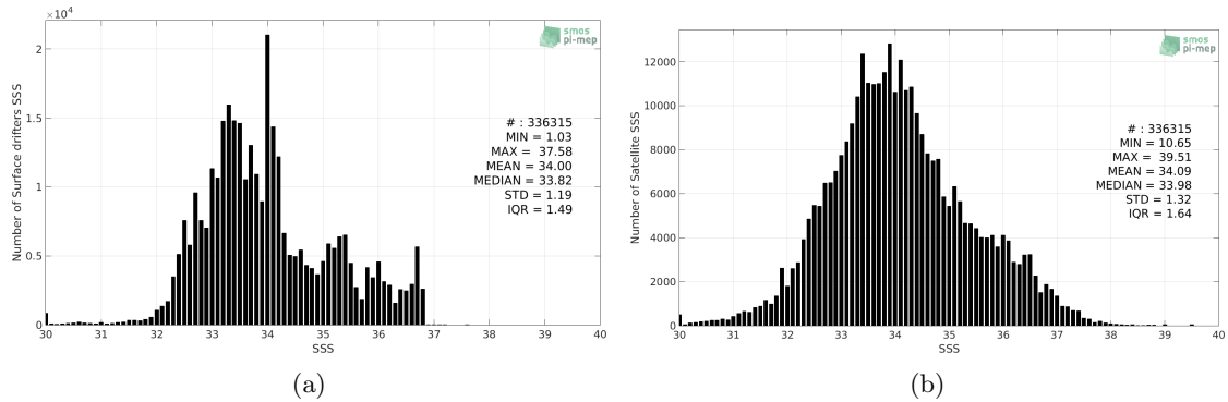
Figure 2: Histograms of SSS from Surface drifters (a) and SMOS SSS L2 v662 (ESA) (b) considering all match-up pairs per bins of 0.1 over the Pacific Ocean Pi-MEP region and for the full satellite product period.
