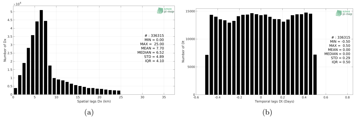
Figure 4: Histograms of the spatial (a) and temporal (b) lags between the time of the Surface drifters measurements and the date of the corresponding SMOS SSS L2 v662 (ESA) SSS product.
