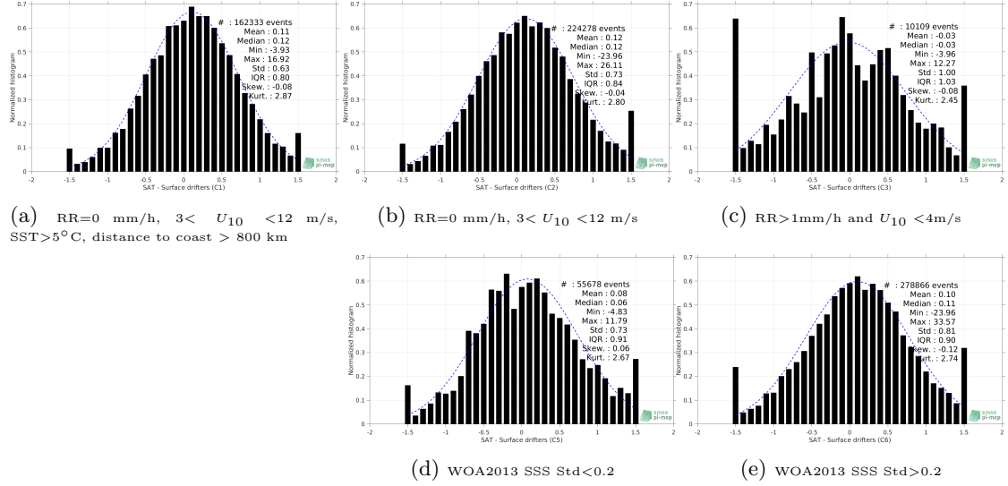
Figure 12: Normalized histogram of \Delta SSS (SMOS L2 v662 (ESA) - Surface drifters) for 5 different subdatasets corresponding to: RR=0 mm/h, 3 < U_{10} < 12 m/s, SST > 5°C, distance to coast > 800 km (a), RR=0 mm/h, 3 < U_{10} < 12 m/s (b), RR > 1mm/h and U_{10} < 4 m/s (c), WOA2013 SSS Std < 0.2 (d), WOA2013 SSS Std > 0.2 (e).
