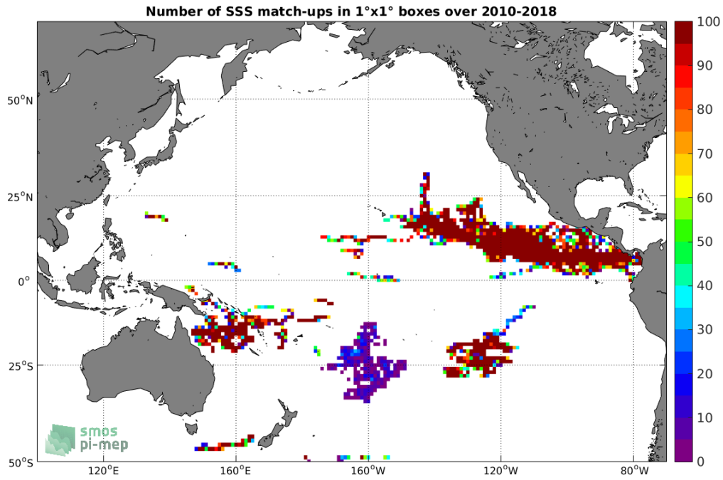
Figure 3: Number of SSS match-ups between Surface drifters SSS and the SMOS L2 v662 (ESA) SSS product for the Pacific Ocean Pi-MEP region over 1^\circ \times 1^\circ boxes and for the full satellite product period.
