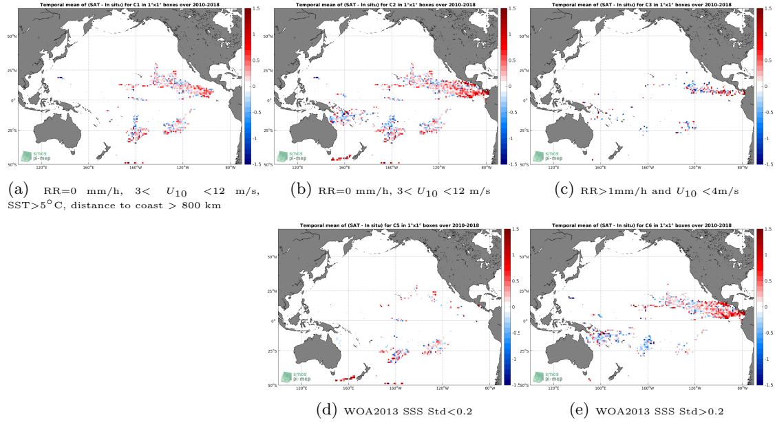
Figure 11: Temporal mean gridded over spatial boxes of size 1^\circ \times 1^\circ of \Delta SSS (SMOS L2 v662 (ESA) - Surface drifters) for 5 different subdatasets corresponding to: RR=0 mm/h, 3 < U_{10} < 12 m/s, SST > 5^\circ C , distance to coast > 800 km (a), RR=0 mm/h, 3 < U_{10} < 12 m/s (b), RR > 1 mm/h and U_{10} < 4 m/s (c), WOA2013 SSS Std < 0.2 (d), WOA2013 SSS Std > 0.2 (e).
