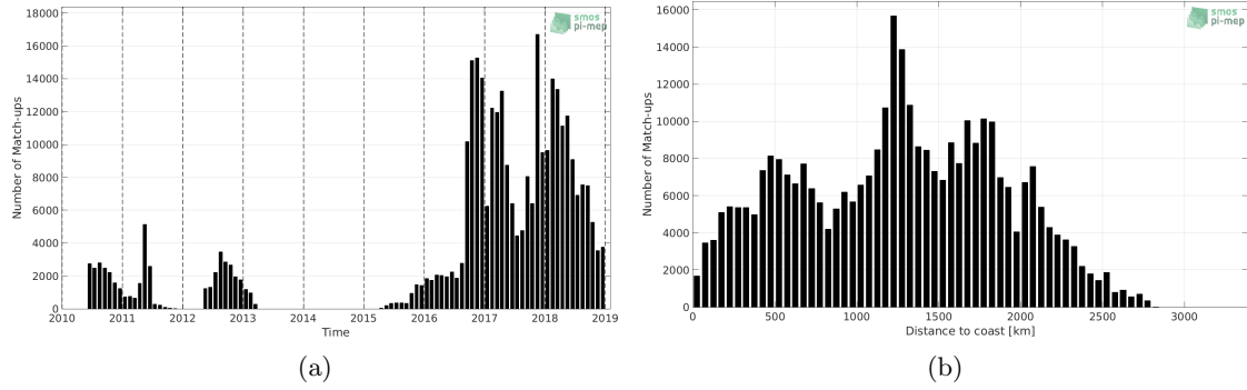
Figure 1: Number of match-ups between Surface drifters and SMOS L2 v662 (ESA) SSS as a function of time (a) and as function of the distance to coast (b) over the Pacific Ocean Pi-MEP region and for the full satellite product period.
