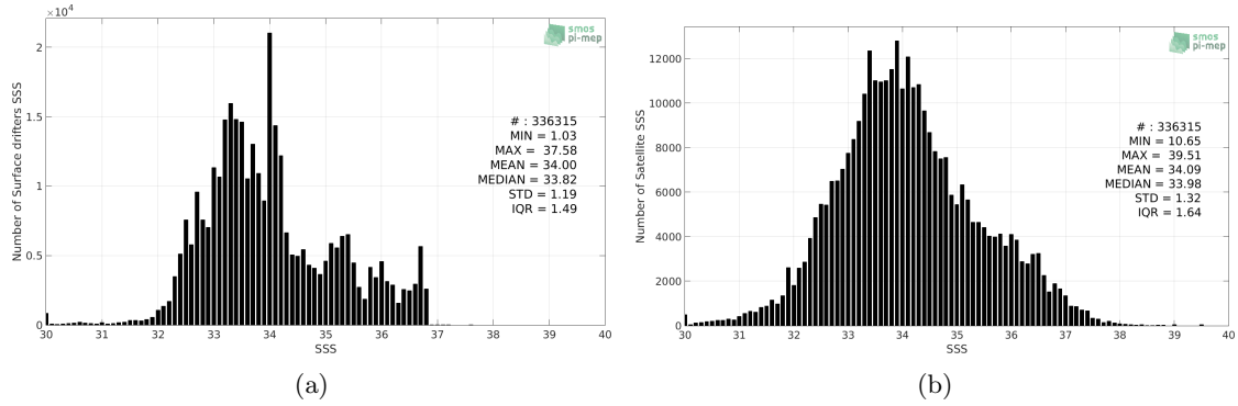
Figure 2: Histograms of SSS from Surface drifters (a) and SMOS L2 v662 (ESA) (b) considering all match-up pairs per bins of 0.1 over the Pacific Ocean Pi-MEP region and for the full satellite product period.
