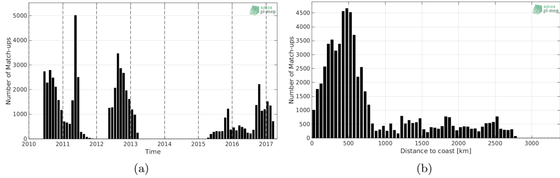
Figure 1: Number of match-ups between Surface drifters and SMOS-L2-DPGS-v662 SSS as a function of time (a) and as function of the distance to coast (b) over the Pacific Ocean Pi-MEP region and for the full satellite product period.
