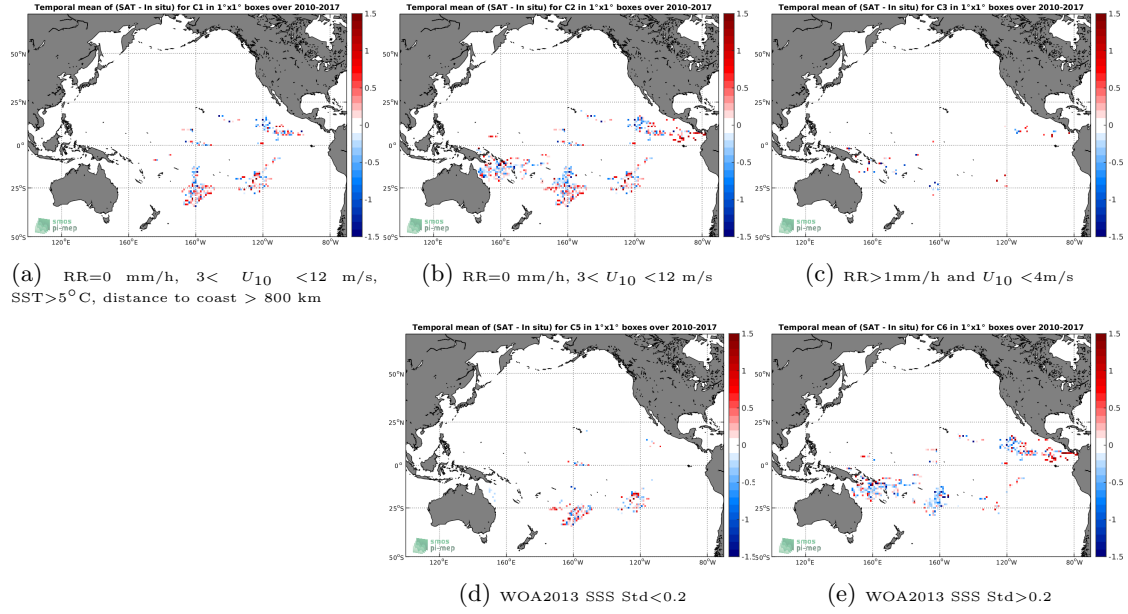
Figure 11: Temporal mean gridded over spatial boxes of size 1^\circ \times 1^\circ of \Delta SSS (SMOS-L2-DPGS-v662 - Surface drifters) for 5 different subdatasets corresponding to: RR=0 mm/h, 3 < U_{10} < 12 m/s, SST >5^\circ C, distance to coast > 800 km (a), RR=0 mm/h, 3 < U_{10} < 12 m/s (b), RR >1 mm/h and U_{10} < 4 m/s (c), WOA2013 SSS Std <0.2 (d), WOA2013 SSS Std >0.2 (e).
