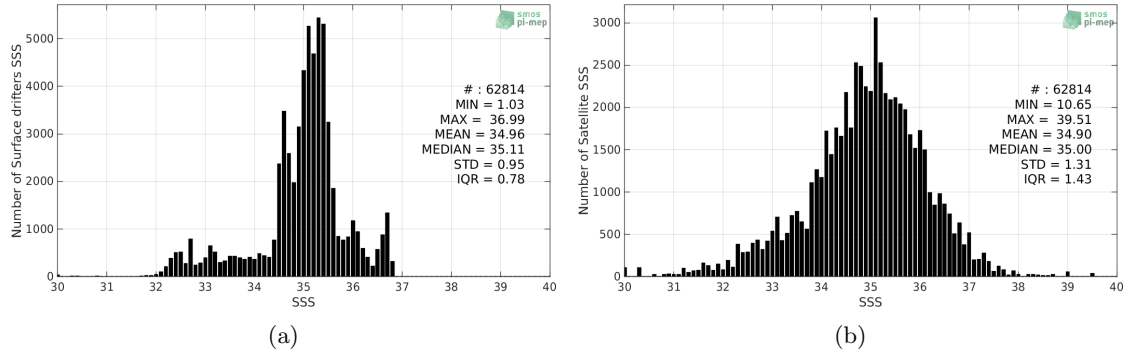
Figure 2: Histograms of SSS from Surface drifters (a) and SMOS-L2-DPGS-v662 (b) considering all match-up pairs per bins of 0.1 over the Pacific Ocean Pi-MEP region and for the full satellite product period.
