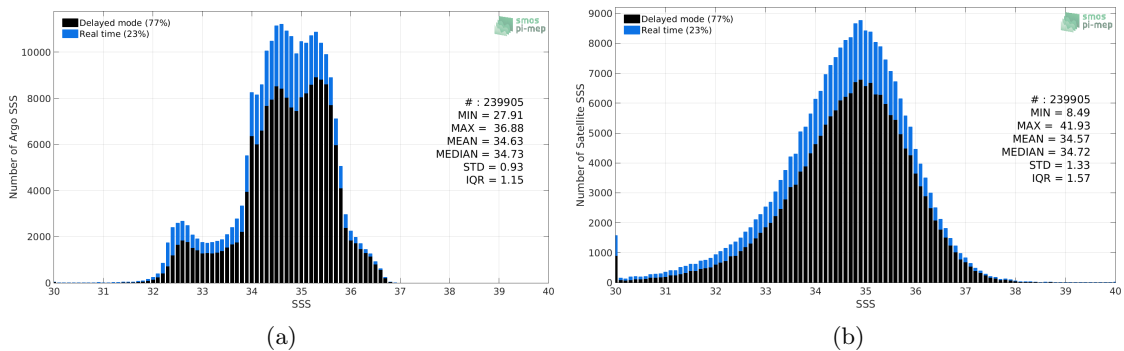
Figure 2: Histograms of SSS from Argo (a) and SMOS L2 v662 (ESA) (b) considering all match-up pairs per bins of 0.1 over the Pacific Ocean Pi-MEP region and for the full satellite product period.
