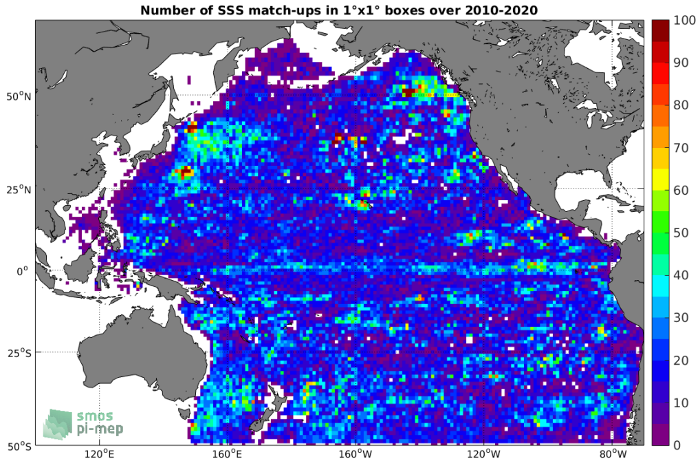
Figure 4: Number of SSS match-ups between Argo SSS and the SMOS L2 v662 (ESA) SSS product for the Pacific Ocean Pi-MEP region over 1^\circ \times 1^\circ boxes and for the full satellite product period.
