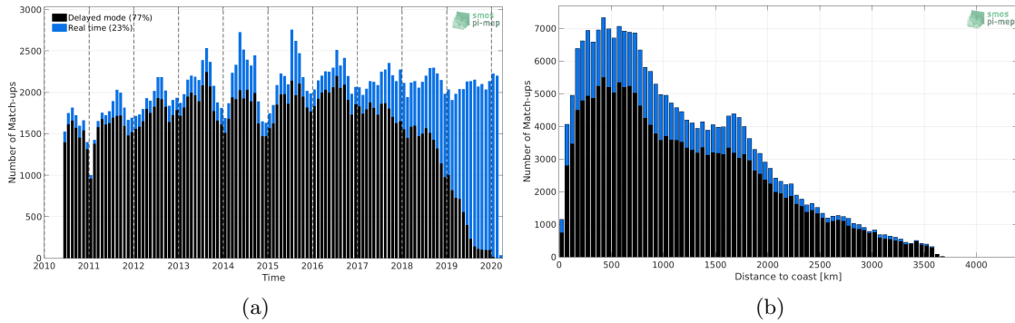
Figure 1: Number of match-ups between Argo and SMOS L2 v662 (ESA) SSS as a function of time (a) and as function of the distance to coast (b) over the Pacific Ocean Pi-MEP region and for the full satellite product period.
