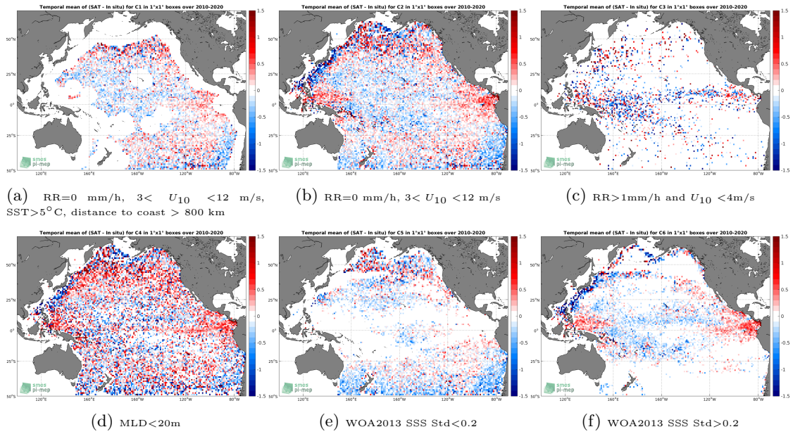
Figure 12: Temporal mean gridded over spatial boxes of size 1^\circ \times 1^\circ of \Delta SSS (SMOS L2 v662 (ESA) - Argo) for 6 different subdatasets corresponding to:RR=0 mm/h, 3 < U_{10} < 12 m/s, SST >5^\circ C, distance to coast > 800 km (a), RR=0 mm/h, 3 < U_{10} < 12 m/s (b), RR >1 mm/h and U_{10} < 4 m/s (c),MLD <20 m (d),WOA2013 SSS Std <0.2 (e),WOA2013 SSS Std >0.2 (f).
