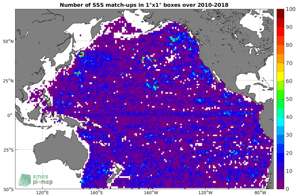
Figure 4: Number of SSS match-ups between Argo SSS and the SMOS-L2-DPGS-v662 SSS product for the Pacific Ocean Pi-MEP region over 1^\circ \times 1^\circ boxes and for the full satellite product period.
