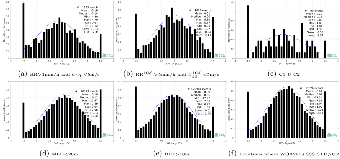
Figure 13: Normalized histogram of \Delta SSS (SMOS-L2-DPGS-v662 - Argo) for 6 different sub-datasets corresponding to: RR > 1\text{mm/h} and U_{10} < 5\text{m/s} (a), RR^{10d} > 5\text{mm/h} and U_{10}^{10d} < 5\text{m/s} (b), C1 \cup C2 (c), MLD < 20\text{m} (d), BLT > 10\text{m} (e), Locations where WOA2013 SSS STD > 0.2 (f).
