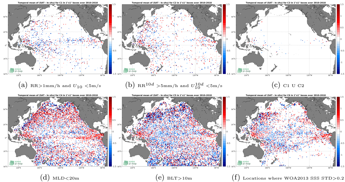
Figure 12: Temporal mean gridded over spatial boxes of size 1^\circ \times 1^\circ of \Delta\text{SSS} (SMOS-L2-DPGS-v662 - Argo) for 6 different subdatasets corresponding to: RR > 1\text{mm/h} and U_{10} < 5\text{m/s} (a), RR^{10d} > 5\text{mm/h} and U_{10}^{10d} < 5\text{m/s} (b), C1 U C2 (c), MLD < 20\text{m} (d), BLT > 10\text{m} (e), Locations where WOA2013 SSS STD > 0.2 (f).
