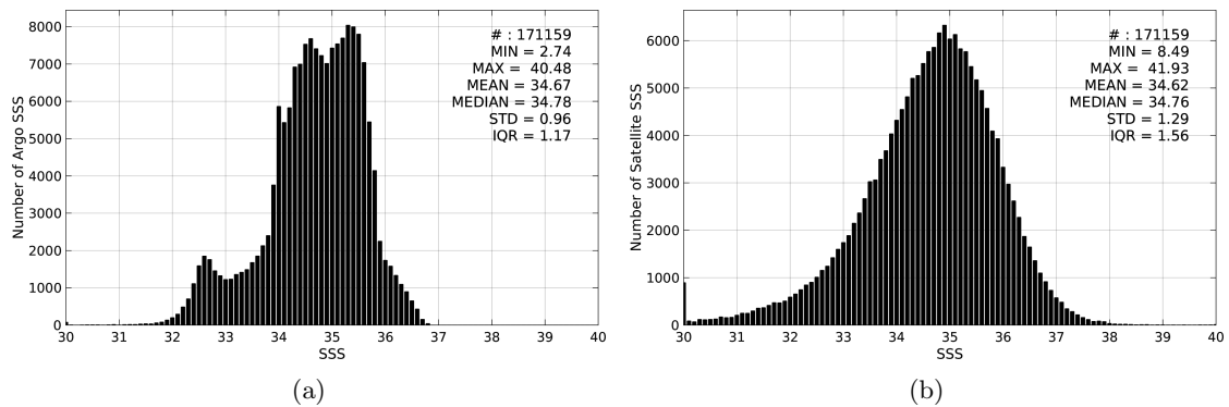
Figure 2: Histograms of SSS from Argo (a) and SMOS-L2-DPGS-v662 (b) considering all match-up pairs per bins of 0.1 over the Pacific Ocean Pi-MEP region and for the full satellite product period.
