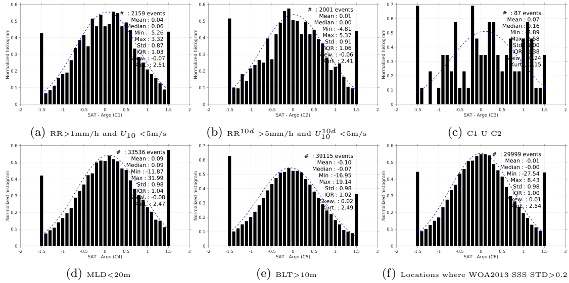
Figure 13: Normalized histogram of \Delta\text{SSS} (SMOS-L2-DPGS-v662 - Argo) for 6 different sub-datasets corresponding to: RR>1mm/h and U_{10} < 5\text{m/s} (a), RR^{10d} > 5\text{mm/h} and U_{10}^{10d} < 5\text{m/s} (b), C1 U C2 (c),MLD<20m (d),BLT>10m (e),Locations where WOA2013 SSS STD>0.2 (f).
