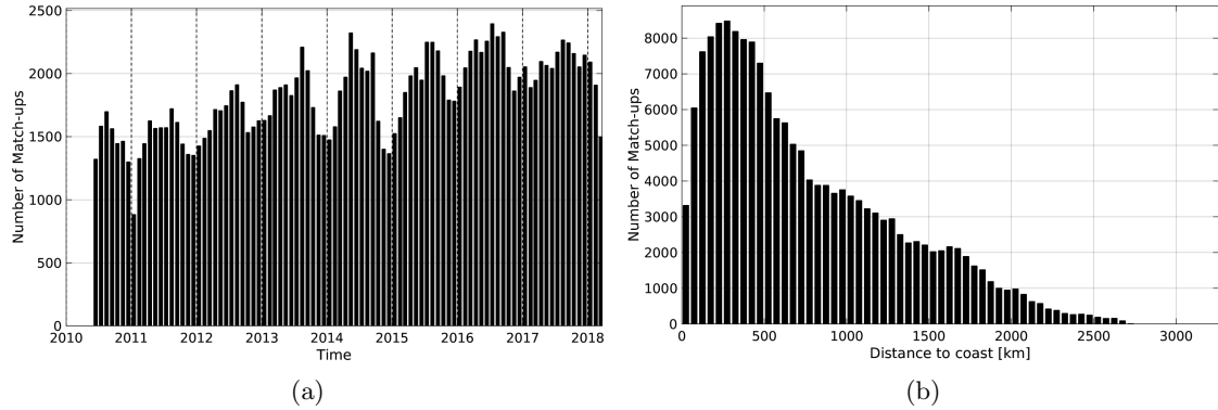
Figure 1: Number of match-ups between Argo and SMOS-L2-DPGS-v662 SSS as a function of time (a) and as function of the distance to coast (b) over the Pacific Ocean Pi-MEP region and for the full satellite product period.
