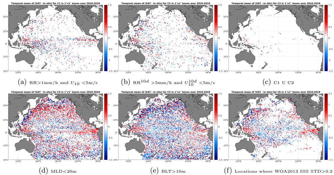
Figure 12: Temporal mean gridded over spatial boxes of size 1^\circ \times 1^\circ of \Delta SSS (SMOS-L2-DPGS-v662 - Argo) for 6 different subdatasets corresponding to: RR > 1mm/h and U_{10} < 5m/s (a), RR^{10d} > 5mm/h and U_{10}^{10d} < 5m/s (b), C1 U C2 (c), MLD < 20m (d), BLT > 10m (e), Locations where WOA2013 SSS STD > 0.2 (f).
