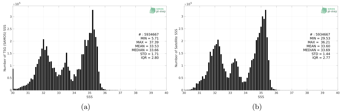
Figure 2: Histograms of SSS from TSG (SAMOS) (a) and SMAP SSS L4 OI v1 - 7 Days (IPRC) (b) considering all match-up pairs per bins of 0.1 over the Pacific Ocean Pi-MEP region and for the full satellite product period.
