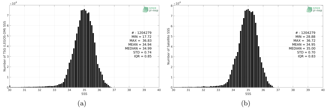
Figure 2: Histograms of SSS from TSG (LEGOS-DM) (a) and SMAP SSS L4 OI v1 - 7 Days (IPRC) (b) considering all match-up pairs per bins of 0.1 over the Pacific Ocean Pi-MEP region and for the full satellite product period.
