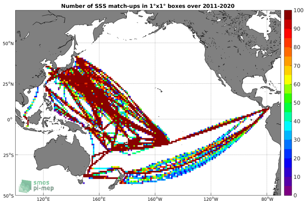
Figure 4: Number of SSS match-ups between TSG (LEGOS-DM) SSS and the SMAP SSS L4 OI v1 - 7 Days (IPRC) SSS product for the Pacific Ocean Pi-MEP region over 1^\circ \times 1^\circ boxes and for the full satellite product period.
